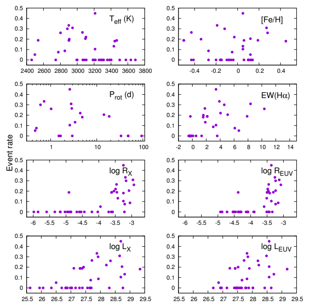
Fig. 3. Line asymmetry rates vs. different physical parameters. EW(H\alpha) , \log R_X and \log R_{EUV} denote H\alpha equivalent width (in Angstroms), and X-ray/EUV activity indices, respectively. \log L_X and \log L_{EUV} plots are in \text{erg s}^{-1} units. Note, that for some objects, some information is missing (e.g. P_{\text{rot}} ), thus not all subplots contain the same number of points.
