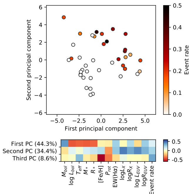
Fig. 5. Result of the principal component analysis (PCA). The top plot shows the data plotted along the first and second principal components. Objects with detected line asymmetries are plotted with filled circles, their shade corresponds to the measured event rate. The bottom plot shows the coefficients for the first three principal components (PCs). The main features of the first PC are related mainly to stellar structure, while the features in the second PC are mainly related to EUV and X-ray activity indices.
