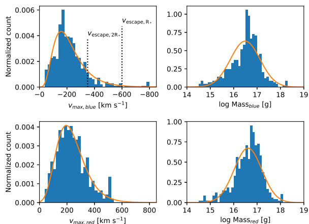
Fig. 7. Distribution of CME velocities and masses from blue and red enhancement. Dashed lines show the approximate escape velocities at the surface and at two stellar radii.
