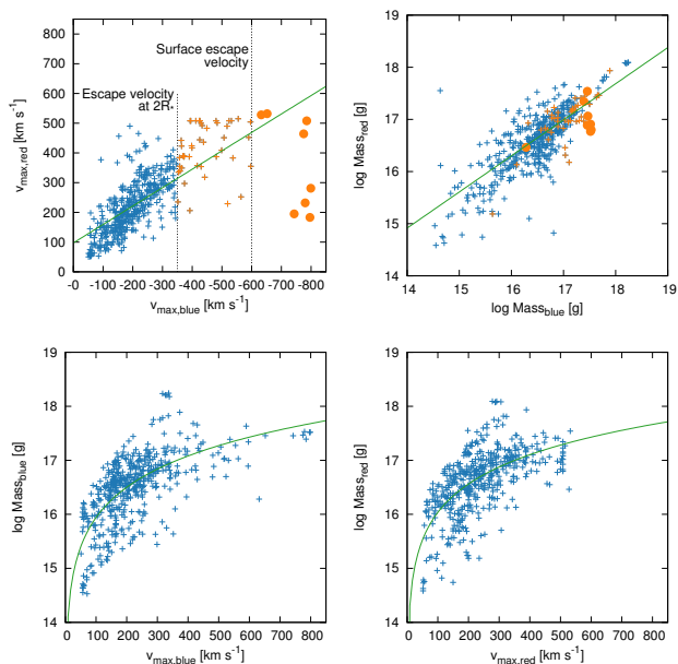
Fig. 6. Top row: Velocities and masses derived from blue vs. red enhancements. On the left plot, vertical lines mark the approximate escape velocity on M dwarfs at the surface and at 2 stellar radii, events with higher speed are marked with different colours on both plots. Lines show linear fits to the data. Bottom row: relation between maximum velocities and estimated masses.
