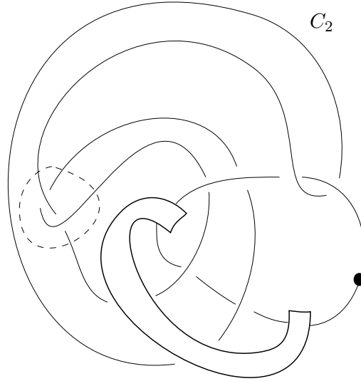
FIGURE 5. After blowing up the clasp in the dashed circle, the two handles will form a cancelling pair, showing that the unknot introduced by the blow-up gives a slice knot in S^3 .
