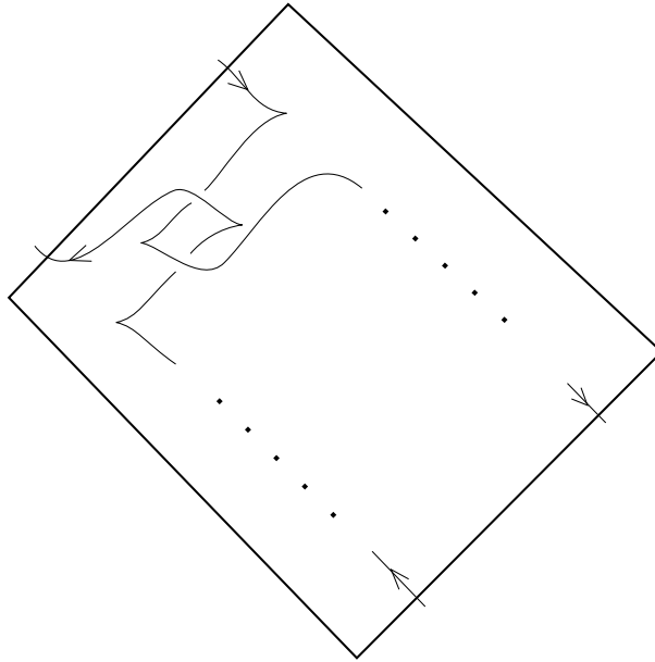
FIGURE 3. The module with n full left twists provides knots K_2(n) with vanishing Thurston-Bennequin numbers. In the diagram the module is already in Legendrian position. Obviously, by adding a left- and a right-cusp to the diagram we get a Legendrian unknot with Thurston-Bennequin number equal to -1 .
