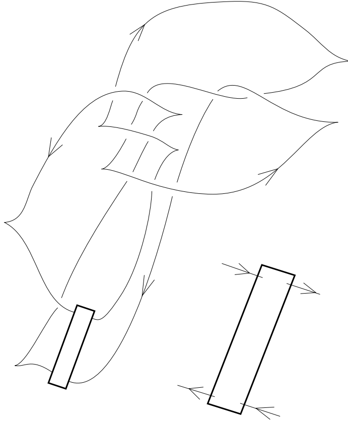
FIGURE 2. The knot K_2 can be isotoped to be the front projection of a Legendrian knot. Indeed, by considering an appropriate modul in the box, the resulting Legendrian knot will have vanishing Thurston-Bennequin number.
