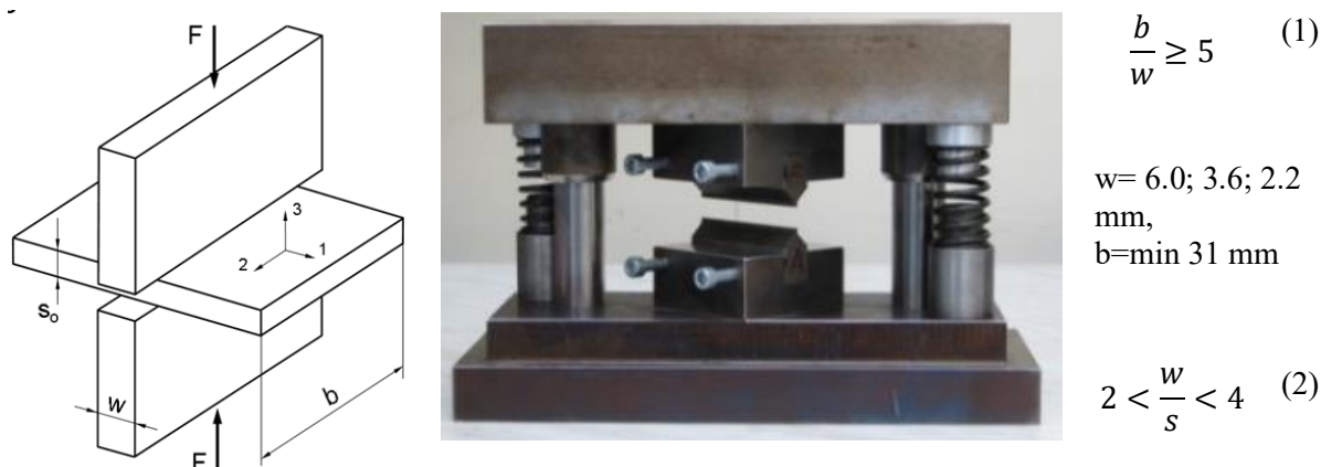
Figure 3. Geometry for Watts-Ford test ( s_0 – initial thickness of specimen, b – initial length of specimen, w – width of dies, F - force) and the inserted die in holder
