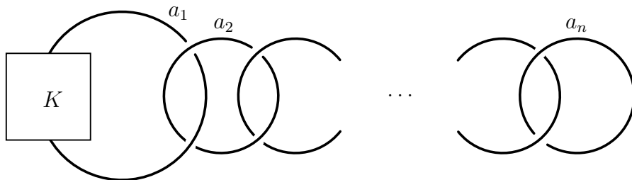
FIGURE 1. The integral surgery picture for p/q -surgery along K , where p/q = [a_1, \dots, a_n]^- .
