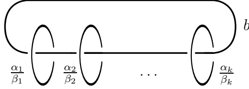
FIGURE 3. A surgery description for the Seifert fibred manifold Y(b; \frac{\alpha_1}{\beta_1}, \dots, \frac{\alpha_k}{\beta_k}) .
