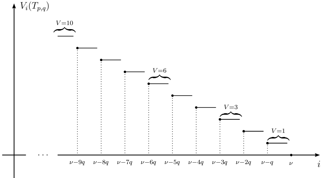
FIGURE 2. A portion of the graph of the function V(\cdot) , under the assumption p > 9q . We let \nu = \nu(T_{p,q}) = \frac{(p-1)(q-1)}{2} .
