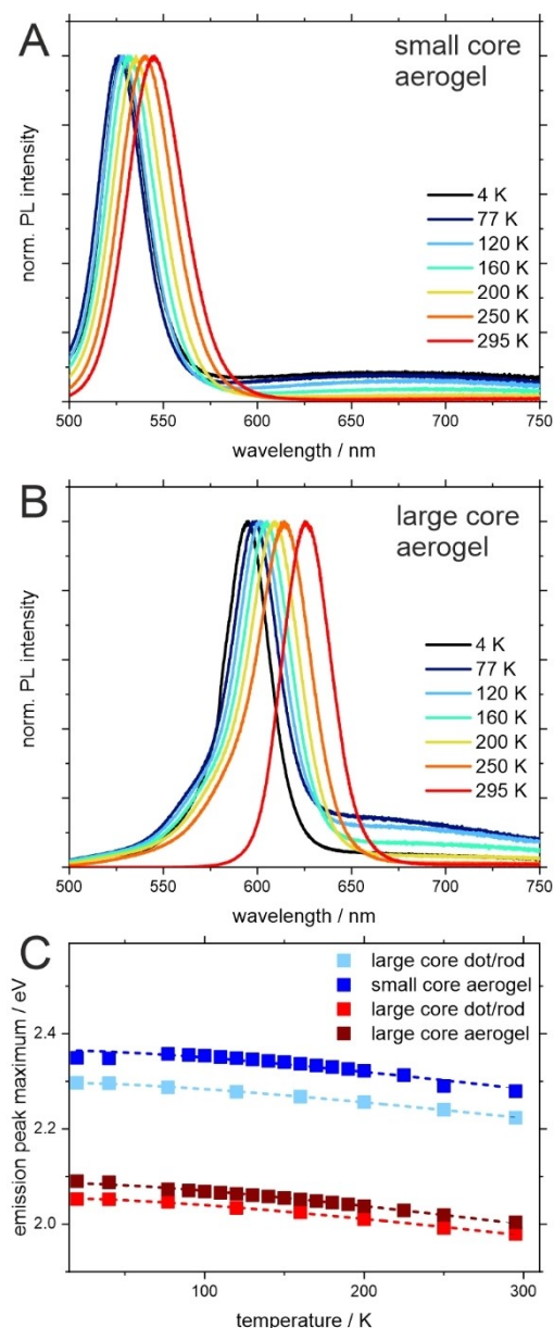
Figure 3. Change of PL with temperature. Temperature dependent emission spectra of CdSe/CdS dot/rod NC-based aerogel networks with (A) CdSe core diameter of 2.0 nm and (B) CdSe core diameter of 3.9 nm. (C) Change in emission maxima depending on temperature and Varshni law fit for CdSe/CdS dot/rod NC-based network structures with different CdSe core sizes (blue colors for small cores, red colors for large cores) and the respective individual building blocks.
