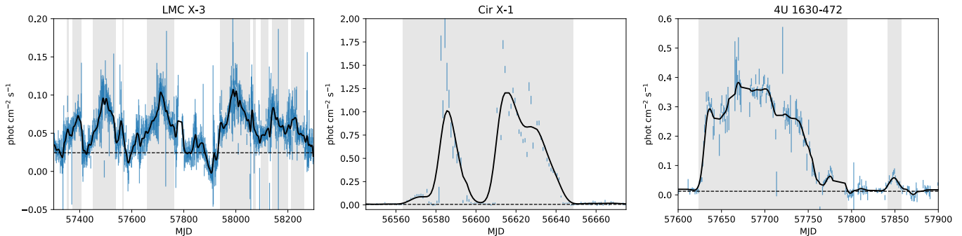
Figure 1. Flare intervals identified from three example light curves. The raw 2-4 keV light curves supplied by the MAXI website (blue) are smoothed with a 3-day Gaussian kernel (black). After subtracting a baseline flux value, identified using the lower 1\text{-}\sigma value of the dataset (dashed black line), intervals with signal-to-noise greater than three are flagged as flares (shaded grey regions). For X-ray binaries that rarely stay quiescent, such as LMC X-3 (left), any bright state is flagged as a flare. Two dust-echo producing flares from Cir X-1 (middle) and 4U 1630-47 (right) are highlighted. The calculated fluences are consistent with those reported in the literature.
