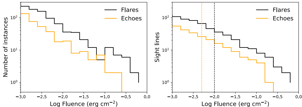
Figure 3. Left: A histogram of flares found in 213 MAXI light curves shows the fluence of the flares themselves (black) and the estimated fluence of the corresponding dust echo (orange). Right: The number of sight lines that exhibit a flare (black) or dust echo (orange) larger than a particular fluence, described on the horizontal axis. This represents the number of sight lines available for performing dust echo tomography. The vertical dashed lines mark the threshold for flares (black) and corresponding echo brightness (orange) above which dust echoes from Galactic XRBs have been observed today. 34 and 24 of the sight lines satisfy two thresholds, respectively.
