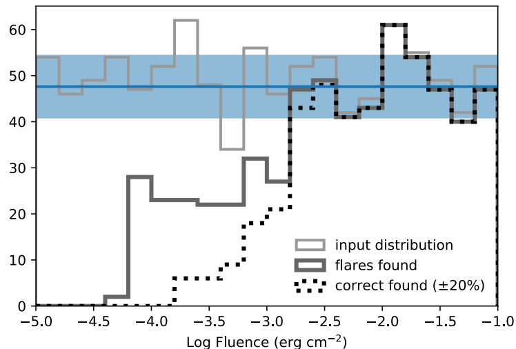
Figure 2. A histogram of simulated input (light grey) and the histogram derived with the techniques described in Section 2 (dark grey). The input flares were drawn from a uniform distribution, and the expected 1\sigma variation is shaded in blue. The dotted black histogram shows how many of the output flares were correct identifications, to within 20% of the input fluence.
