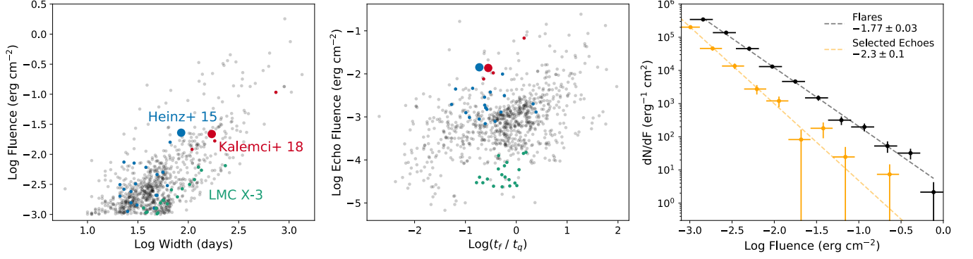
Figure 4. Left: Relationship between flare duration and 2-4 keV fluence of the flare, as measured by MAXI. Naturally, the larger fluence flares tend to arise from longer duration flares, up to 1000 days. The blue, red, and green circles show data points from the flares observed from Cir X-1, 4U 1630-47, and LMC X-3, respectively. The flares that led to dust echoes studied by Heinz et al. (2015) and Kalemci et al. (2018) are highlighted by the large blue and red circles, respectively. Middle: Plot of the dust echo 2-4 keV fluence versus the ring sharpness metric, ( t_f/t_q ). The larger fluence flares, which are often longer, are less useful because they fill out more of the dust scattering halo and produce broad rings that are more likely to overlap. The Cir X-1, 4U 1630-47, and LMC X-3 flares are highlighted in the same way as the left plot (blue, red, and green). In general, flares with ( t_f/t_q ) \ll 1 produce the most ideal dust echoes for high resolution dust echo tomography. Right: A power law fit to the fluence distribution for all flares (black) and dust echoes with t_q/t_f < 1 (orange) yields power law slopes of -1.77 \pm 0.03 and -2.3 \pm 0.1 , respectively.
