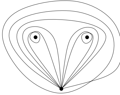
Fig. 1. A non-homotopic loose multigraph with 3 vertices and 6 edges, all of which are loops.
