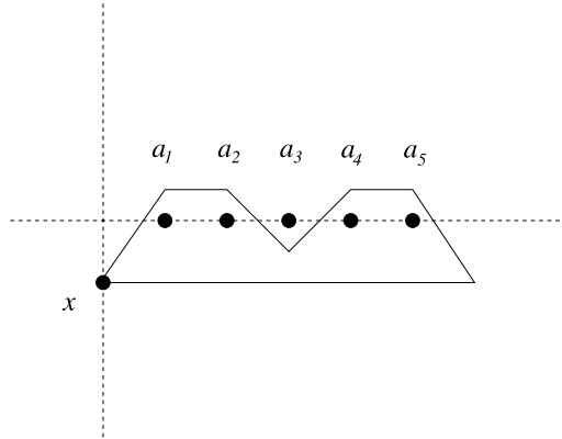
Fig. 3. An elementary x -loop ( n = 5 ).
