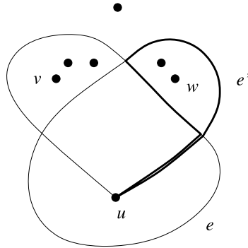
Fig. 2. The replacement of e by e' in the proof of Lemma 7.
