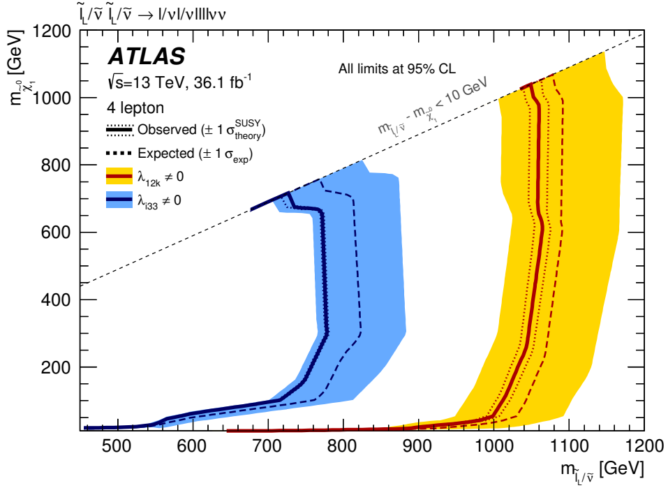
(a) RPV \tilde{\ell}_L/\tilde{\nu} NLSP
