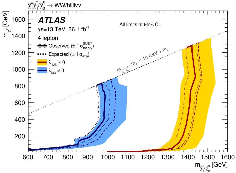
Figure 7: Expected (dashed) and observed (solid) 95% CL exclusion limits on (a) wino W/Z NLSP, and (b) wino W/h NLSP pair production with RPV \tilde{\chi}_1^0 decays via \lambda_{12k} , or \lambda_{133} where i, k \in 1, 2 . The limits are set using the statistical combination of disjoint signal regions. Where the signal regions are not mutually exclusive, the observed CL_s value is taken from the signal region with the better expected CL_s value.
