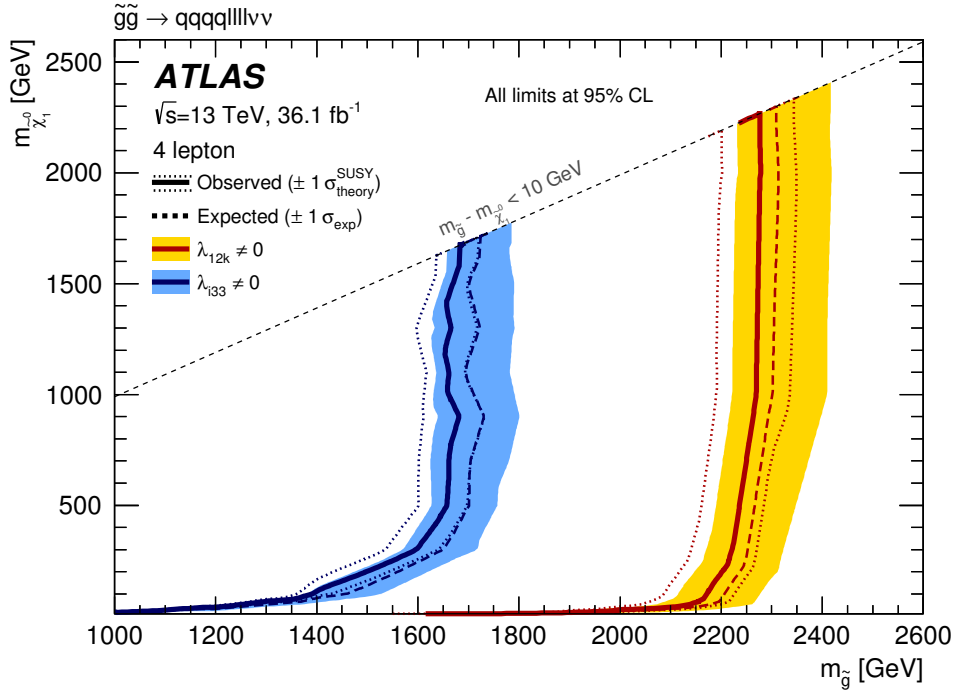
(b) RPV \tilde{g} NLSP
