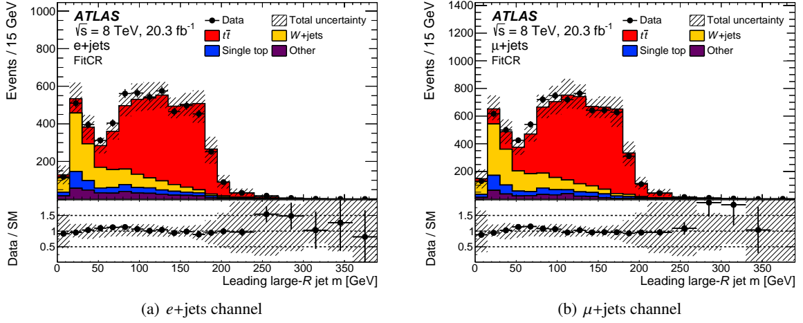
Figure 3: Comparison of data to the expected background for the leading large- R jet mass in the FitCR, both for the electron (left) and muon (right) channels, after applying the W +jets and t\bar{t} normalisation correction factors.
