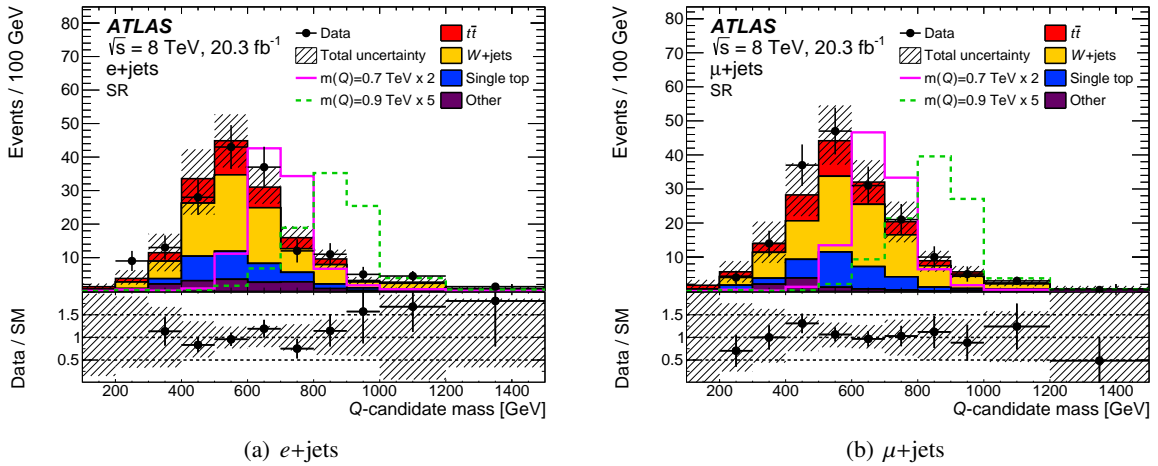
Figure 4: Distribution of the Q -candidate mass for the electron and muon channels before the likelihood fit. The signal yields are shown for cross-sections corresponding to c_L^{Wb} = 1 and for \text{BR}(Q \rightarrow Wb) = 0.5 . These are scaled up, in order to improve their visibility. The uncertainty band includes all the uncertainties listed in Section 8, which are taken as fully uncorrelated between different sources.
