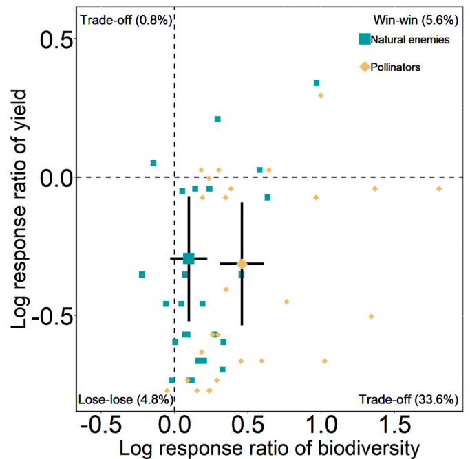
Fig. 2. Scatter plot of log response ratio between biodiversity and yield in agri-environment scheme vs control fields on croplands. Presented are species richness mean effect size by functional groups (natural enemies and pollinators) with 95 % CIs. Effects are significant if the CI lines do not cross zero lines. The points represent raw data values based on the studied functional groups. % indicates the percentage of the dataset (for abundance, see Fig. S3 ). The percentages in the plot indicate the proportions of effect size combinations in the four scenarios.
