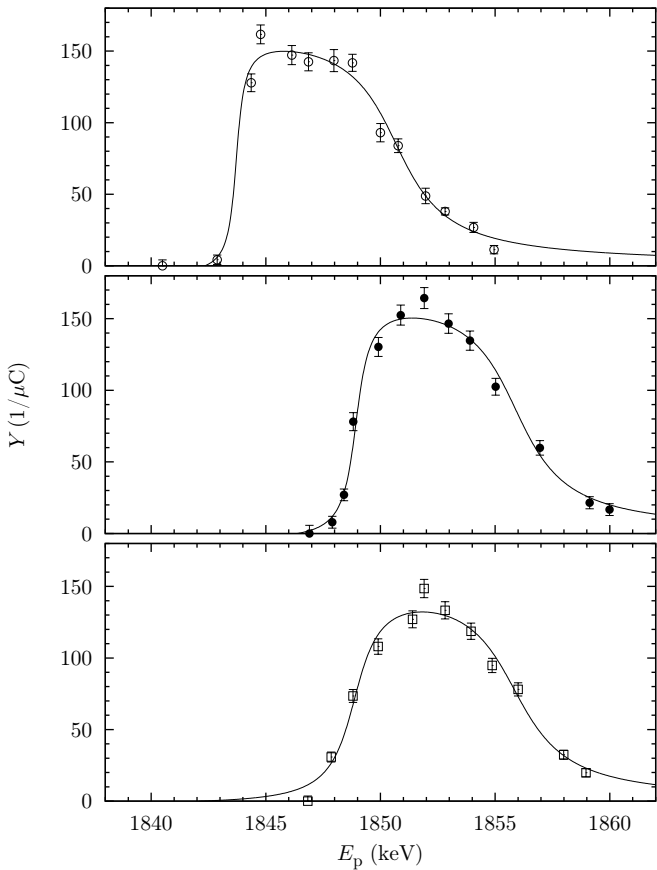
FIG. 1. Experimental yield of the 2882 keV \gamma ray in target #31 scans before first (open circles), between first and second (closed circles), and after second (open squares) part of the \alpha -beam irradiation, as a function of proton beam energy. Lines are results of fits using Eq. (7). The proton energy shift in the two lower panels is due to an impurity layer buildup on the target. This layer also increases the beam energy straggling, which is seen by somewhat flatter slopes.
