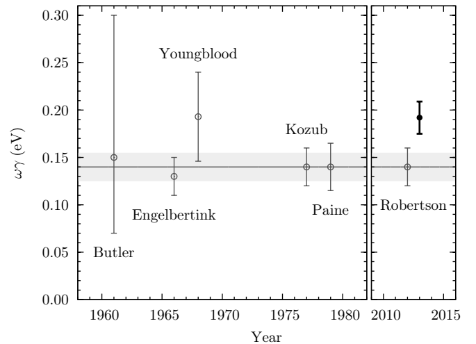
FIG. 2. Literature data (open circles), compared with the present result (filled circle). The previously evaluated value [3, 17] is given as a horizontal shaded bar.
