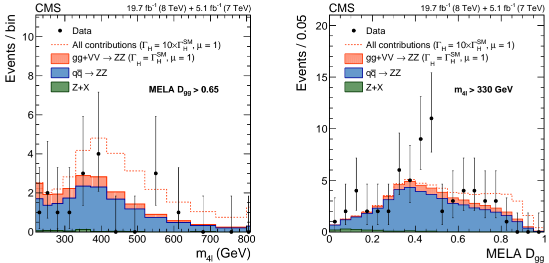
Figure 3: Distributions of (left) the four-lepton invariant mass after a selection requirement on the MELA likelihood discriminant \mathcal{D}_{\text{gg}} > 0.65 , and (right) the \mathcal{D}_{\text{gg}} likelihood discriminant for m_{4\ell} > 330 GeV in the 4\ell channel. Points represent the data, filled histograms the expected contributions from the reducible (Z+X) and q\bar{q} backgrounds, and from the gluon fusion (gg) and vector boson fusion (VV) SM processes (including the Higgs boson mediated contributions). The dashed line corresponds to the total expected yield for a Higgs boson width and a squared product of the couplings scaled by a factor 10 with respect to their SM values. In the top plot, the bin size varies from 20 to 85 GeV and the last bin includes all entries with masses above 800 GeV.
