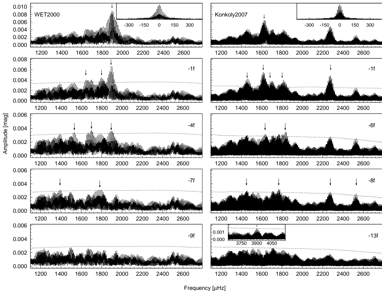
Fig. 3. Successive pre-whitening steps of the analyses of the WET2000 and Konkoly2007 datasets. The window functions are given in the inserts. Dashed lines denote the 4\langle A \rangle significance levels calculated by the moving average of the spectra.
