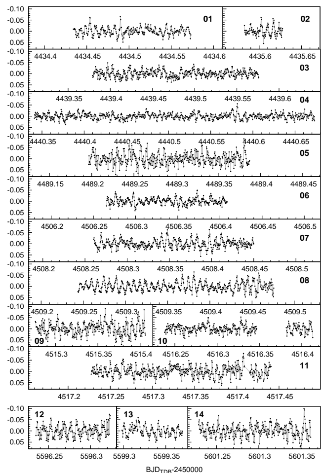
Fig. 2. Normalized differential light curves of the Konkoly runs. Data were collected in the 2007/2008 observing season (upper panels) and in 2011 (lower panels), respectively. For the better visibility of the pulsation cycles, we connected the points with grey lines. Boldface numbers in the corners correspond to the run numbers in Table 1.
