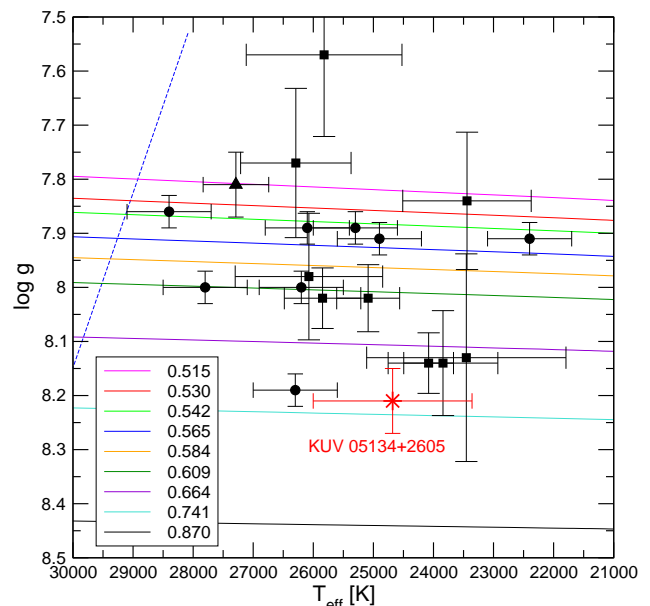
Fig. 7. The location of the known DBV stars on the T_{\text{eff}} - \log g plane. Also included are our DB white dwarf evolutionary tracks displayed with different colours according to the stellar mass. The location of KUV 05134+2605 as given by spectroscopy is emphasized with a red asterisk symbol. The theoretical blue edge of the DBV instability strip corresponding to the version MLT2 ( \alpha = 1.25 ) of the MLT theory of convection, as derived by Córscico et al. (2009b), is depicted with a blue dashed line.
