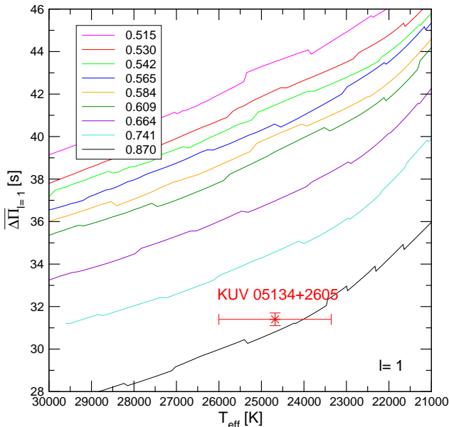
Fig. 8. The average of the computed period spacings for \ell = 1 corresponding to our DB white dwarf sequences with different stellar masses. The location of KUV 05134+2605 is shown with a red asterisk symbol ( T_{\text{eff}} = 24\,700 \pm 1\,300 K) for the observed \Delta\Pi_{\ell=1} = 31.4 \pm 0.3 solution of mean period spacing. By simple linear interpolation, we found that the mass of the star according to its period spacing is M_* = 0.85 \pm 0.05 M_{\odot} .
