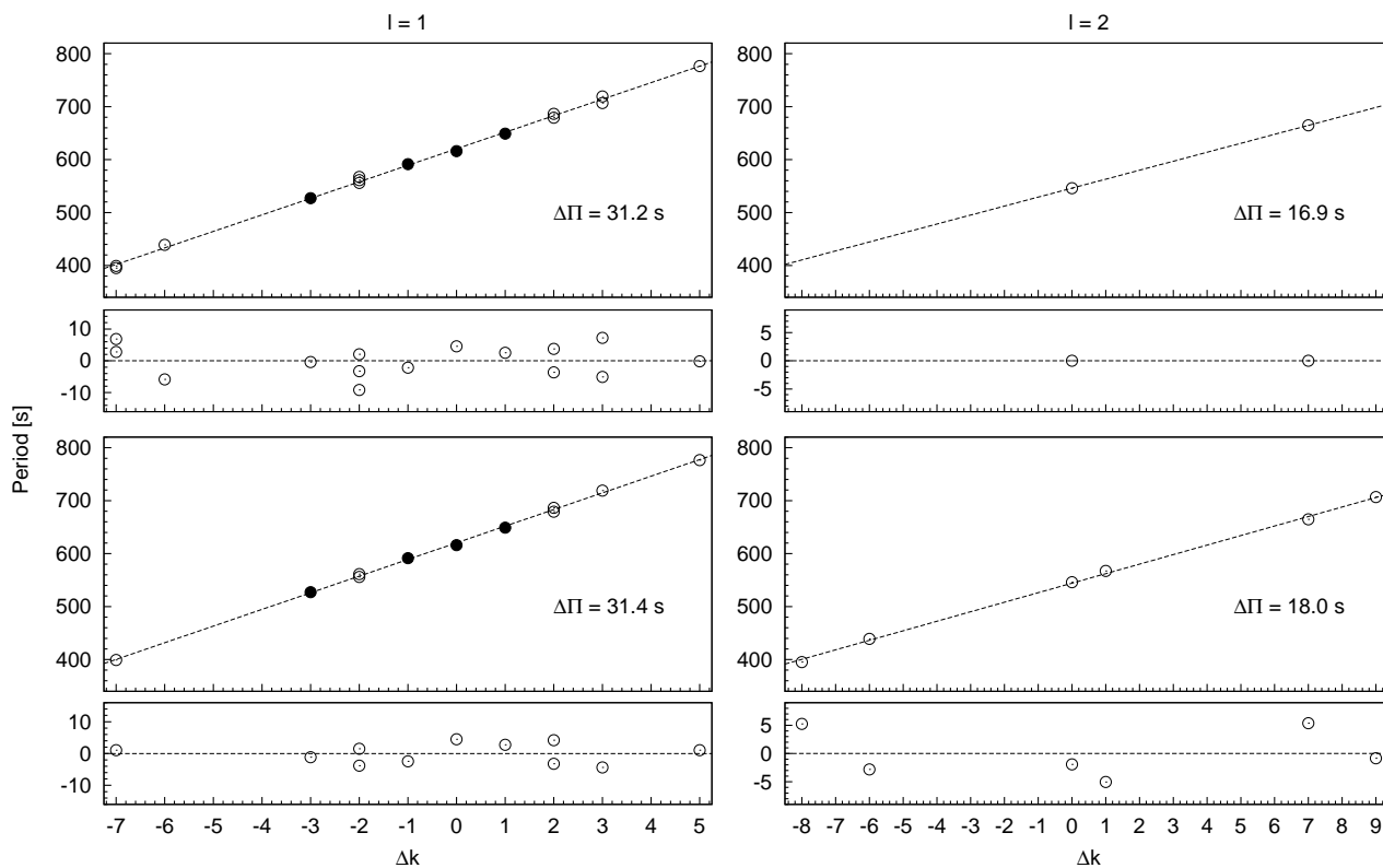
Fig. 4. Periods of Table 4 plotted in the \Delta k – period planes. Filled circles denote average periods by the 9 \mu\text{Hz} spacings. The panels on the left and right show the \ell = 1 and 2 solutions and their linear least-squares fits, respectively. The residuals of the fits are also presented. Top and bottom rows display different solutions by changing some periods' presumed \ell values. The resulting period spacings ( \Delta\Pi_{\ell=1,2} ) are denoted.
