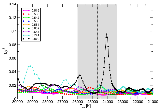
Fig. 9. The inverse of the quality function of the period fit in terms of the effective temperature for Case 3 . The vertical grey strip indicates the spectroscopic T_{\text{eff}} and its uncertainties ( T_{\text{eff}} = 24\,700 \pm 1300 K).
