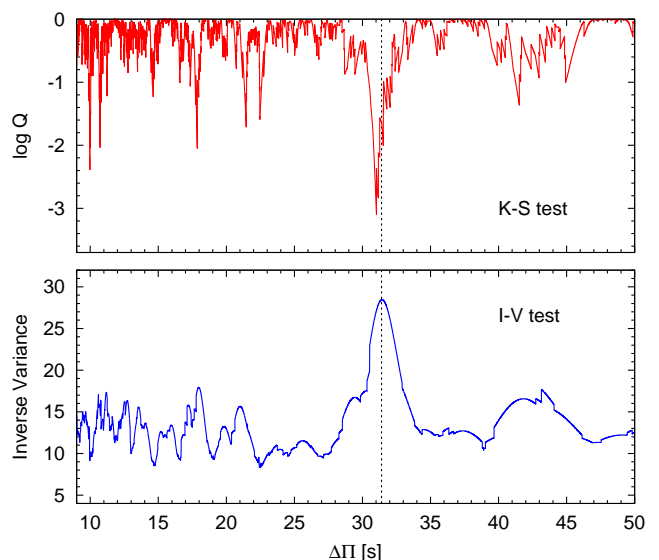
Fig. 5. Characteristic spacings of the periods listed in Table 4, applying the Kolmogorov-Smirnov (K-S) and the Inverse Variance (I-V) significance tests. The vertical dotted line denotes the 31.4 s spacing value obtained in Sect. 3.4.2.
