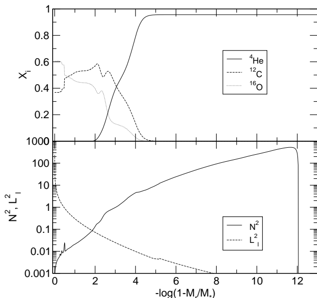
Fig. 11. The internal chemical structure (upper panel), and the squared Brunt-Vaisala and Lamb frequencies for \ell = 1 (lower panel) corresponding to our best-fit DB white dwarf model with a stellar mass M_* = 0.84 M_\odot , an effective temperature T_{\text{eff}} = 25\,050\text{ K} , and a He envelope mass of M_{\text{He}}/M_* \sim 1.5 \times 10^{-3} .
