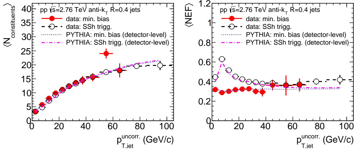
Fig. 77: Mean total number of constituents (left) and mean neutral energy fraction (right) measured in reconstructed jets in 2.76 TeV pp collisions (anti-kT, R = 0.4 ), vs. jet p_T . Data are shown for MB and SSh triggers, and are compared to detector-level simulations.
