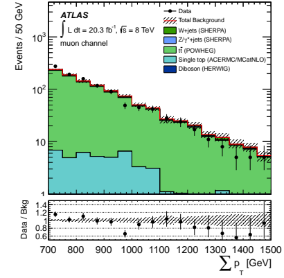
(f) t\bar{t} CR, \sum p_T , muon channel.
