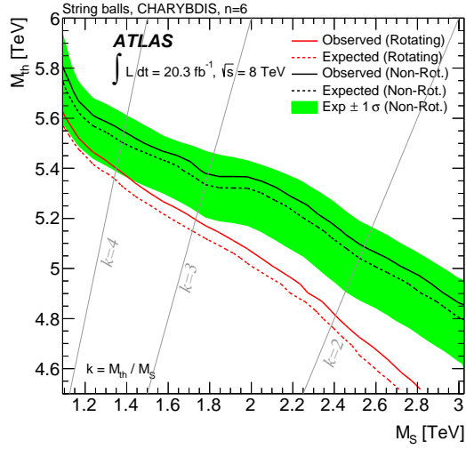
Figure 9. The exclusion limits in the M_{th} – M_S plane, with electron and muon channels combined, for rotating and non-rotating string ball models with six extra dimensions. The solid (dashed) lines show the observed (expected) 95% CL limits, with the band illustrating the expected \pm 1\sigma variation of the expected limits for the non-rotating case. The \pm 1\sigma variation is comparable for the rotating case. Masses below the corresponding lines are excluded. The lighter grey lines indicate constant k = M_{th}/M_S .
