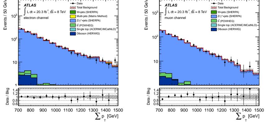
(a) Z +jets CR, \sum p_T , electron channel.
