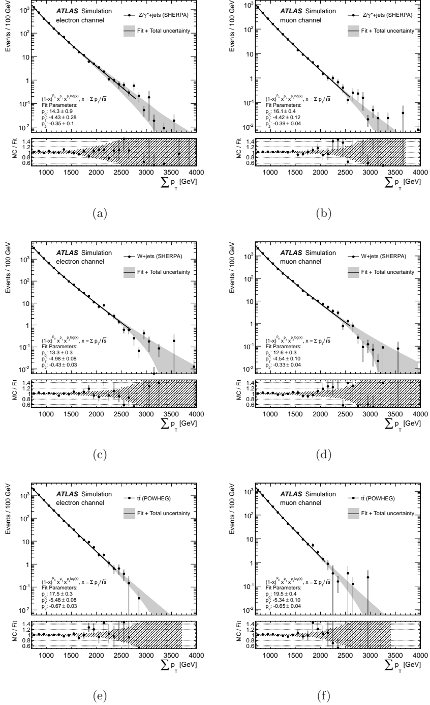
Figure 4. The \sum p_T distributions and fit curves for (a, b) Z+\gamma +jets; (c, d) W +jets (+ diboson); and (e, f) t\bar{t} (+ single-top) MC-simulated events. Distributions for the electron channel are on the left while those for the muon channel are on the right. The shaded bands on the fit curves reflect the total uncertainty on the fit, including the systematic uncertainty discussed in section 7.3. The length of the black line indicates the \sum p_T range fitted. The lower panels show the ratio of the MC prediction to the fit, with the statistical uncertainty on the MC prediction (points), and separately, the fractional uncertainty on the fit (shaded band).
