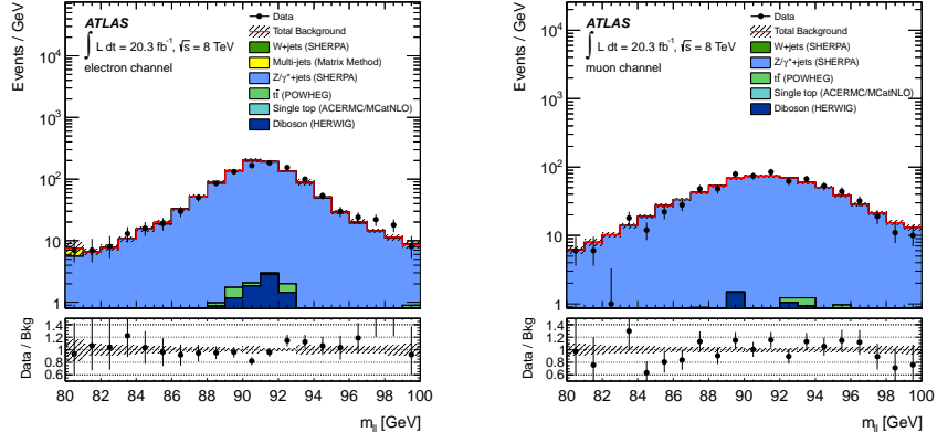
(a) Z +jets CR, dilepton invariant mass, (b) Z +jets CR, dilepton invariant mass, electron channel, muon channel.
