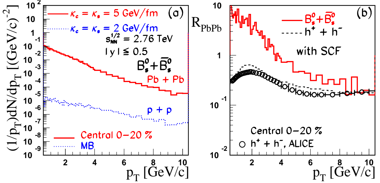
FIG. 7: (Color online) Part (a): HIJING/BB v2.0 predictions for p_T distributions at mid-rapidity for \text{Pb} + \text{Pb} \rightarrow (B_s^0 + \bar{B}_s^0)/2 + X (upper histogram), and for p + p collisions (lower histogram). Part (b): The p_T dependence of NMF R_{AA}(p_T) for B_s^0 mesons (solid histogram) and charged particles (dashed histogram) in central (0-20%) \text{Pb} + \text{Pb} collisions. Data are from ALICE Collaboration for charged particles (open circles) [121]. Error bars include only statistical uncertainties.
