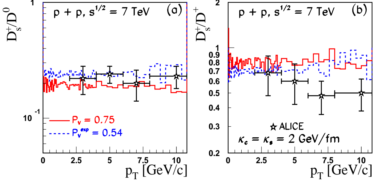
FIG. 9: (Color online) Comparison of HIJING/BB v2.0 predictions for ratios of strange D_s^+ to non-strange mesons D^0 (left panel) and D^+ (right panel). The histograms have the same meaning as in Fig. 8. The data are from Refs. [73], [74]. Error bars include only the statistical uncertainty.
