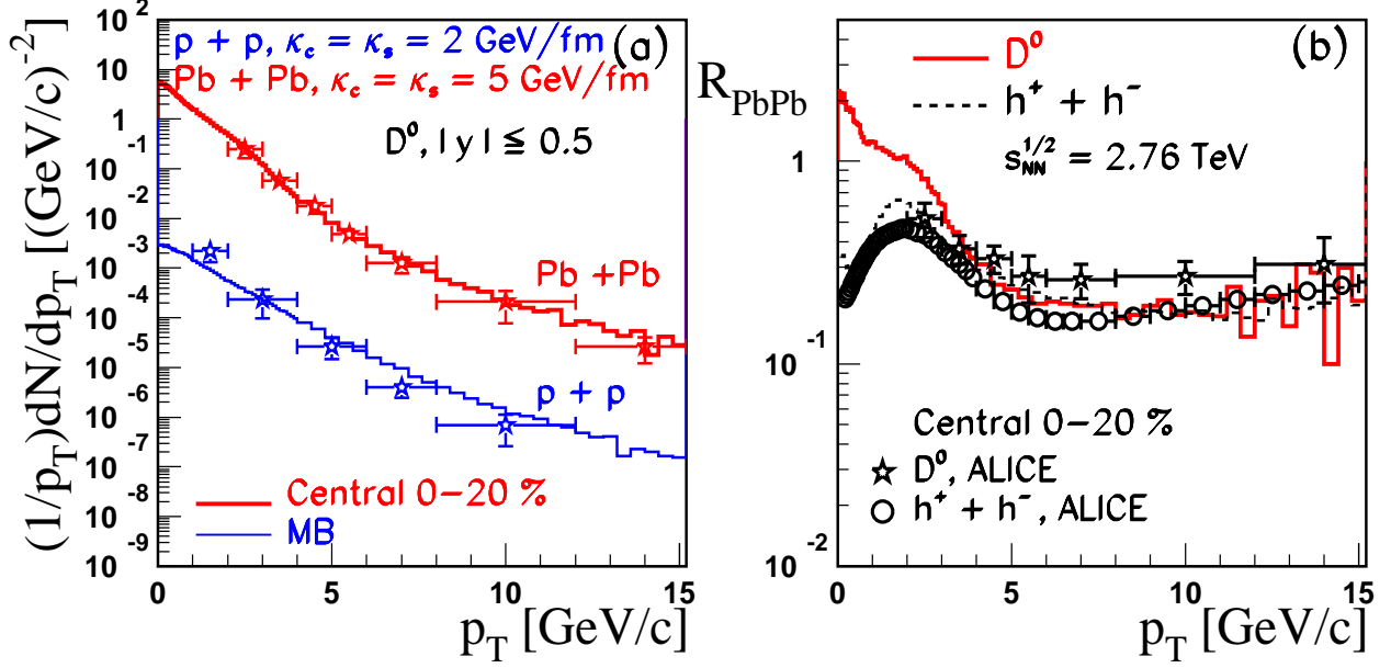
FIG. 2: (Color online) Part (a): HIJING/BB v2.0 predictions for p_T distributions at mid-rapidity for \text{Pb} + \text{Pb} \rightarrow (D^0 + \bar{D}^0)/2 + X (upper histogram), and for p + p collisions (lower histogram). Part (b): The p_T dependence of NMF R_{\text{AA}}(p_T) for D^0 mesons (solid histogram) and charged particles (dashed histogram) in central (0-20 %) \text{Pb} + \text{Pb} collisions. Data are from ALICE Collaboration for D^0 (stars) [79] and for charged particles (open circles) [121]. Error bars include only statistical uncertainties.
