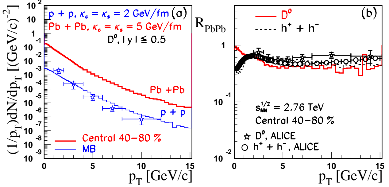
FIG. 3: (Color online) Comparison of HIJING/BB v2.0 predictions of p_T distributions (left panel) and NMF R_{AA}(p_T) for D^0 and charged particles in semi-peripheral (40-80 %) Pb + Pb collisions (right panel). The histograms have the same meaning as in Fig. 2. Data are from ALICE Collaboration for D^0 (stars) [79] and for charged particles (open circles) [121]. Error bars include only the statistical uncertainties.
