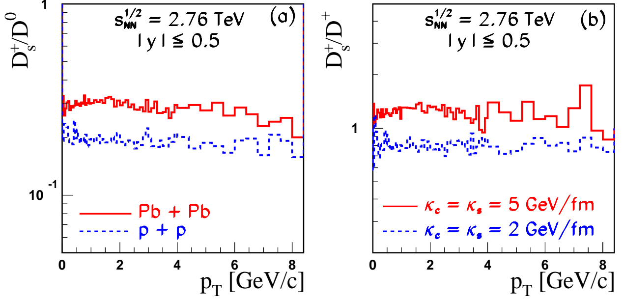
FIG. 10: (Color online) Comparison of HIJING/ B\bar{B} v2.0 predictions for ratios of strange D_s^+ to non-strange mesons D^0 (left panel) and D^+ (right panel) at \sqrt{s} = 2.76 TeV in p + p collisions and at \sqrt{s_{NN}} = 2.76 TeV in centrality class 0-20 % in Pb+Pb collisions. The results are shown for \kappa_c = \kappa_s = 2 GeV/fm (dashed histogram) and for in medium value \kappa_c = \kappa_s = 5 GeV/fm (solid histograms). The parameter P_V is set at its default value P_V = 0.75 .
