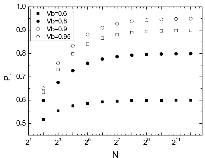
FIG. 8. The achievable maximal single-photon probability P_1 at the optimal choice \lambda_{\text{opt}}^{(N)} of the mean photon pair number as a function of the number N of multiplexed units on semi-logarithmic scale for different generic transmission coefficients V_b for an ideal multiplexer, and assuming ideal detectors ( V_D = 1 ).
