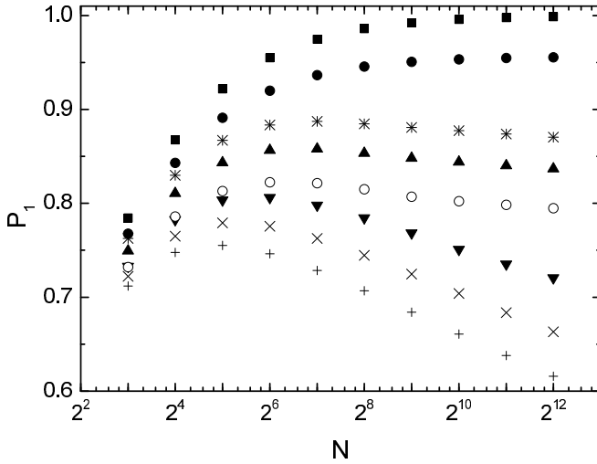
FIG. 18. The achievable maximal single-photon probability P_1 at the optimal choice \lambda_{\text{opt}}^{(N)} of the mean photon pair number as a function of the number of time windows N on semi-logarithmic scale for various loss coefficients for the proposed bulk time multiplexer, assuming ideal detectors and no generic losses ( V_D = V_b = 1 ). The legend of the symbols is in Tab. II.
