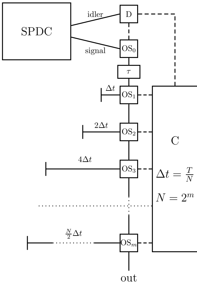
FIG. 3. Periodic photon source. SPDC is a spontaneous parametric down-conversion source yielding twin photon pairs; D: detector unit detecting idler photons and switching OS_0 ; OS_0 is an optical switch with a gate width \Delta t that selects the twin signal photon; C is the controller unit setting the optical switches OS_i ( i = 1, \dots, m ) ensuring proper delay of the twin photon; the delay \tau is needed for the proper operation of the controller C.
