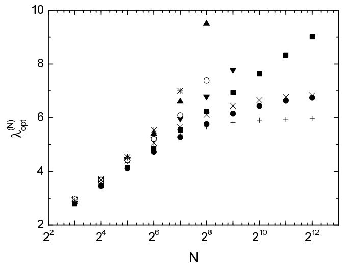
FIG. 17. The optimal choice \lambda_{\text{opt}}^{(N)} of the mean photon pair number as a function of the number of time windows N on semi-logarithmic scale for various loss coefficients for the proposed bulk time multiplexer, assuming ideal detectors and no generic losses ( V_D = V_b = 1 ). The legend of the symbols is in Tab. II.
