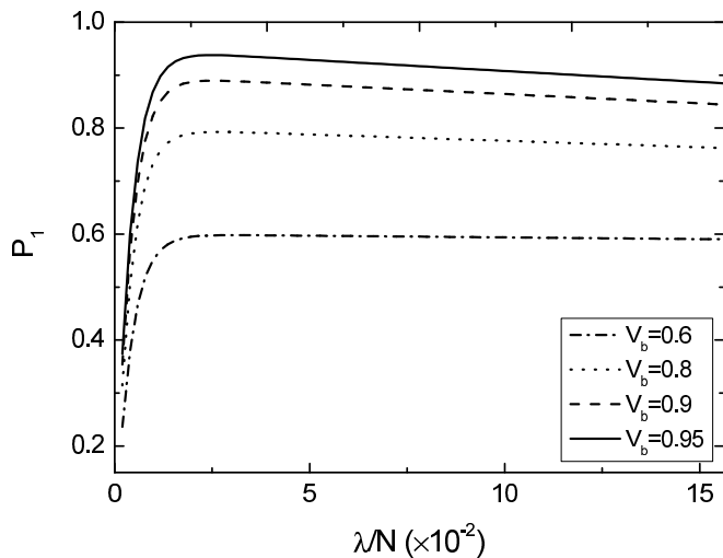
FIG. 5. The single-photon probability P_1 plotted against the mean photon pair number per multiplexed unit \lambda/N for various generic transmission coefficients V_b , considering N = 256 multiplexed units for an ideal multiplexer, and assuming ideal detectors ( V_D = 1 ).
