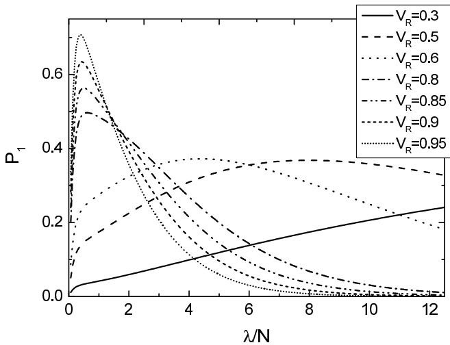
FIG. 9. The single-photon probability P_1 plotted against the mean photon pair number per multiplexed unit \lambda/N , for various router transmission coefficients V_R , considering N = 8 multiplexed units for a spatial multiplexer, assuming ideal detectors and no generic losses ( V_D = V_b = 1 ).
