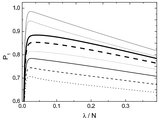
FIG. 16. The single-photon probability P_1 as a function of \lambda/N for different combinations of loss parameters, considering a system of N = 256 time windows, that is, of m = 8 delay units for the proposed bulk time multiplexer, assuming ideal detectors and no generic losses ( V_D = V_b = 1 ). From top to bottom the curves presented in the figure correspond to the transmission values indicated in Tab. II from 1 to 8.
