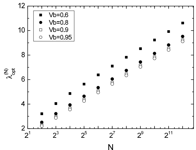
FIG. 7. The optimal choice \lambda_{\text{opt}}^{(N)} of the mean photon pair number as a function of the number of multiplexed units N on semi-logarithmic scale for different generic transmission coefficients V_b for an ideal multiplexer, and assuming ideal detectors ( V_D = 1 ).
