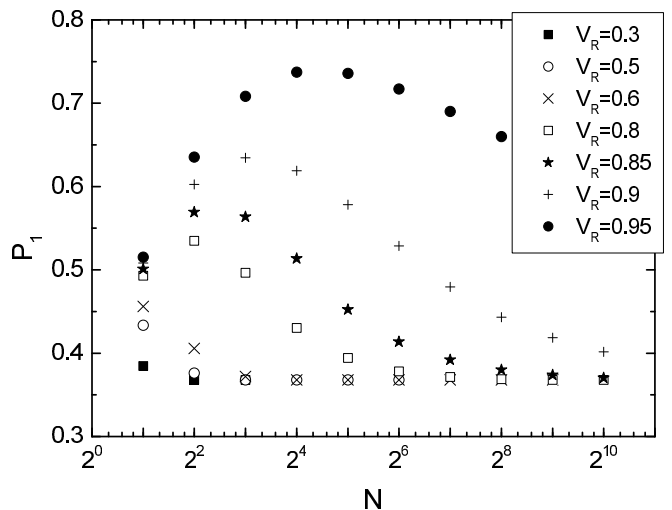
FIG. 11. The achievable maximal single-photon probability P_1 at the mean photon pair number \lambda_{\text{opt}}^{(N)} as a function of the number N of multiplexed units on a semi-logarithmic scale for different router transmission coefficients V_R for a spatial multiplexer, and assuming ideal detectors and no generic losses ( V_D = V_b = 1 ).
