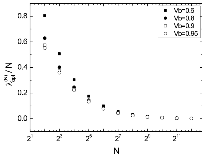
FIG. 6. The optimal choice \lambda_{\text{opt}}^{(N)}/N of the mean photon pair number per multiplexed unit as a function of the number of multiplexed units N on semi-logarithmic scale for different generic transmission coefficients V_b for an ideal multiplexer, and assuming ideal detectors ( V_D = 1 ).
