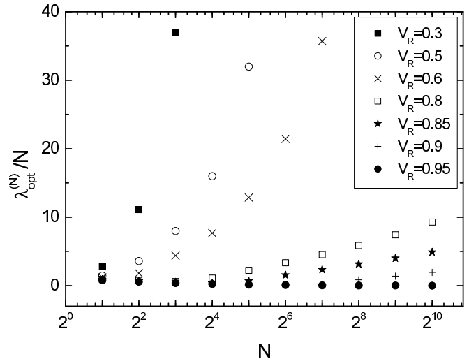
FIG. 10. The optimal choice \lambda_{\text{opt}}^{(N)}/N of the mean photon pair number per multiplexed unit as a function of the number of multiplexed units N on semi-logarithmic scale for different router transmission coefficients V_R for a spatial multiplexer, assuming ideal detectors and no generic losses ( V_D = V_b = 1 ).
