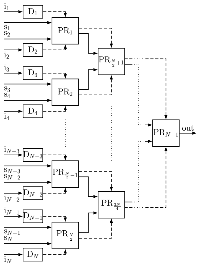
FIG. 1. Schematics of a spatially multiplexed periodic single-photon source. PR_j : j th photon router, the D_j -s are detectors, i_j and s_j are the idler and signal arms of the j th SPDC source. Dashed lines represent electronic control lines.
