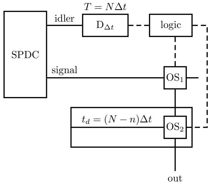
FIG. 2. Schematics of a storage cavity-based periodic photon source. SPDC is a spontaneous parametric down-conversion source yielding twin photon pairs; OS_1 and OS_2 are optical switches. t_d is the delay introduced by the cavity if the idler photon was detected in the n -th time window of length \Delta t within the period of T = N \Delta t .
