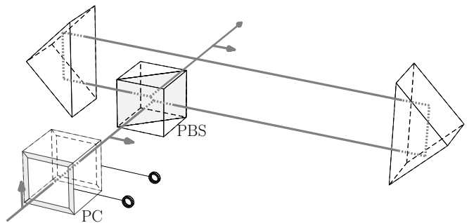
FIG. 4. Schematic figure of a single delay unit. PC: Pockels cell, PBS: polarizing beam splitter. An initially vertically polarized photon arrives at the Pockels cell. By changing its polarization, the photon can be forced to use the delay line.
