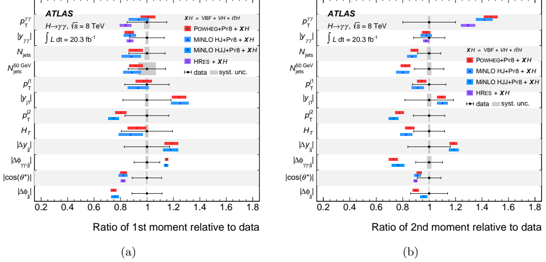
Figure 9. (a) The ratio of the first moment (mean) of each differential distribution predicted by the theoretical models to that observed in the data. (b) The ratio of the second moment (RMS) of each differential distribution predicted by the theoretical models to that observed in the data. The intervals on the vertical axes each represent one of the differential distributions. The band for each theoretical prediction represents the corresponding uncertainty in that prediction (see text for details). The error bar on the data represents the total uncertainty in the measurement, with the grey band representing the systematic-only uncertainty.
