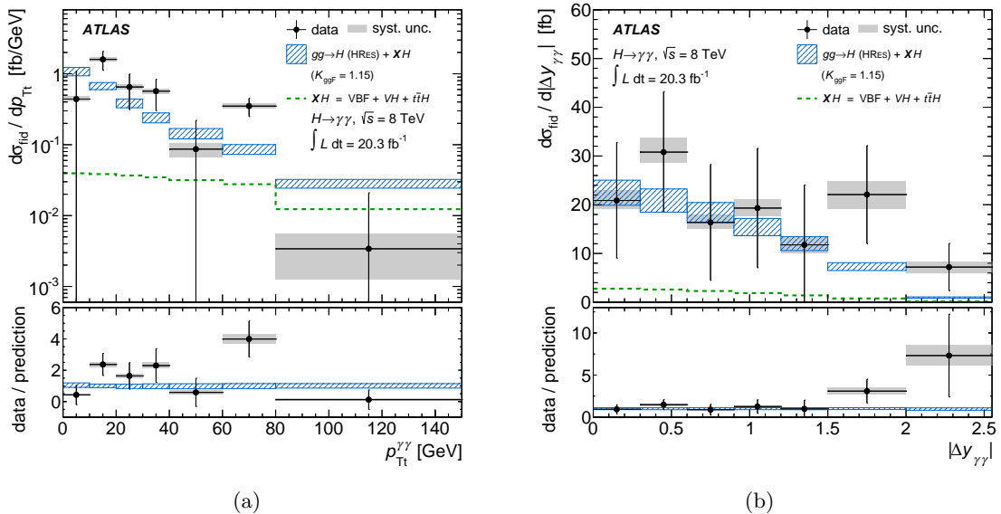
Figure 10. The differential cross section for pp \rightarrow H \rightarrow \gamma\gamma as a function of (a) p_{\text{T}}^{\gamma\gamma} and (b) |\Delta y_{\gamma\gamma}| . The data are shown as filled (black) circles. The vertical error bar on each data point represents the total uncertainty in the measured cross section, and the shaded (grey) band is the systematic uncertainty component. The SM prediction, defined using the HRES prediction for gluon fusion and the default MC samples for the other production mechanisms, is presented as a hatched (blue) band (see text for details). The small contribution from VBF, VH and t\bar{t}H is also shown separately as a dashed (green) line and denoted as XH . The HRES predictions are normalised to the total LHC-XS cross section [57] using a K-factor of K_{\text{ggF}} = 1.15 .
