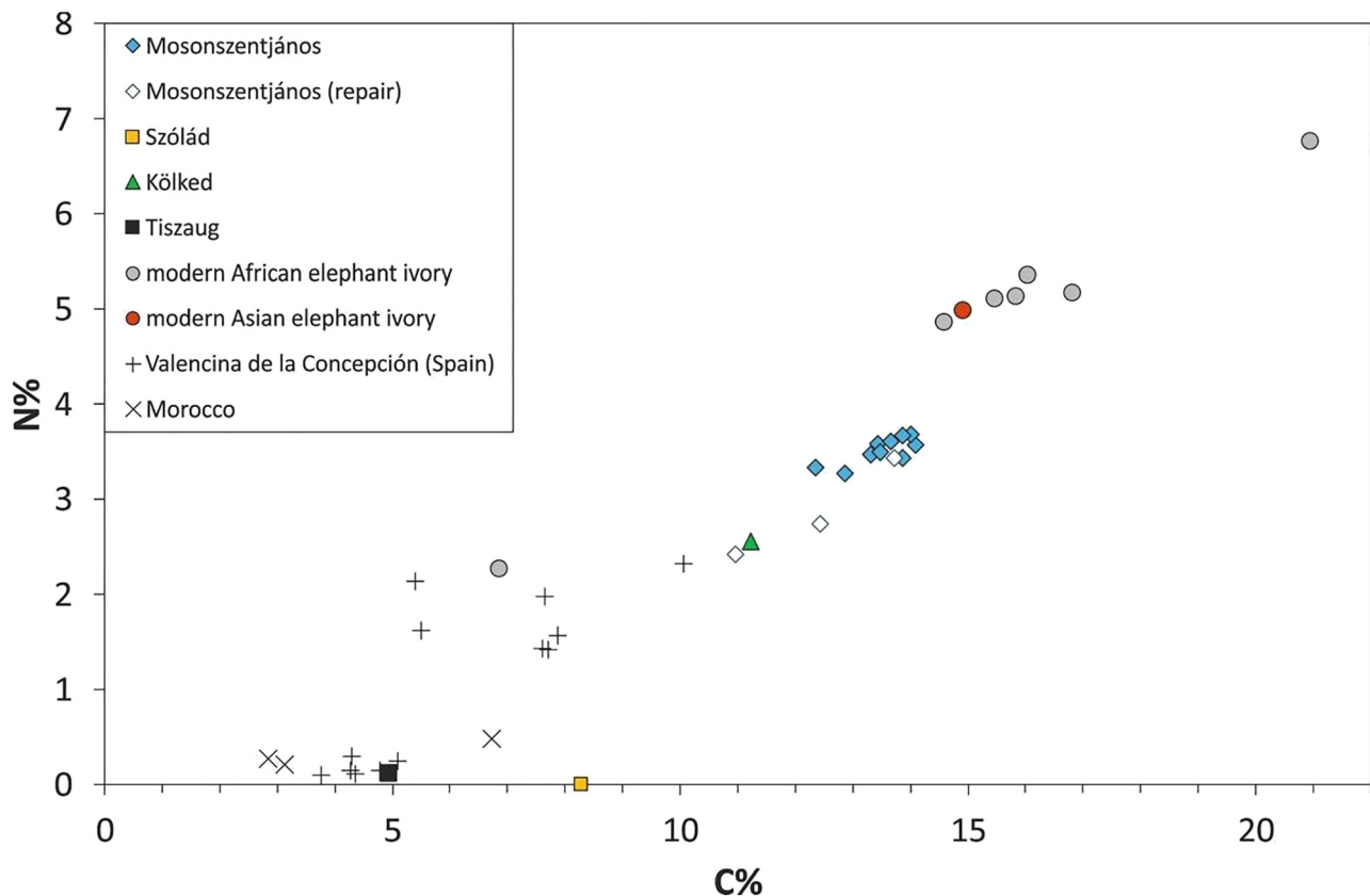
Fig. 7. Nitrogen vs. carbon content of the studied archaeological ivory findings from Mosonszentjános, Szólád, Kölked, and Tiszaug (Inv. numbers beginning with 66 indicate objects from Mosonszentjános, including repairs denoted as 'R' in the sample name). Archaeological ivory objects from Morocco (Banerjee et al., 2011) and Spain (Nocete et al., 2013; García Sanjuán et al., 2013), as well as modern African and Asian ivory pieces from the Mammal Collection of the Hungarian Natural History Museum are indicated for comparison. As the N content of the Szólád sample could not be determined due to small sample size, it is indicated as 0% N in the figure
