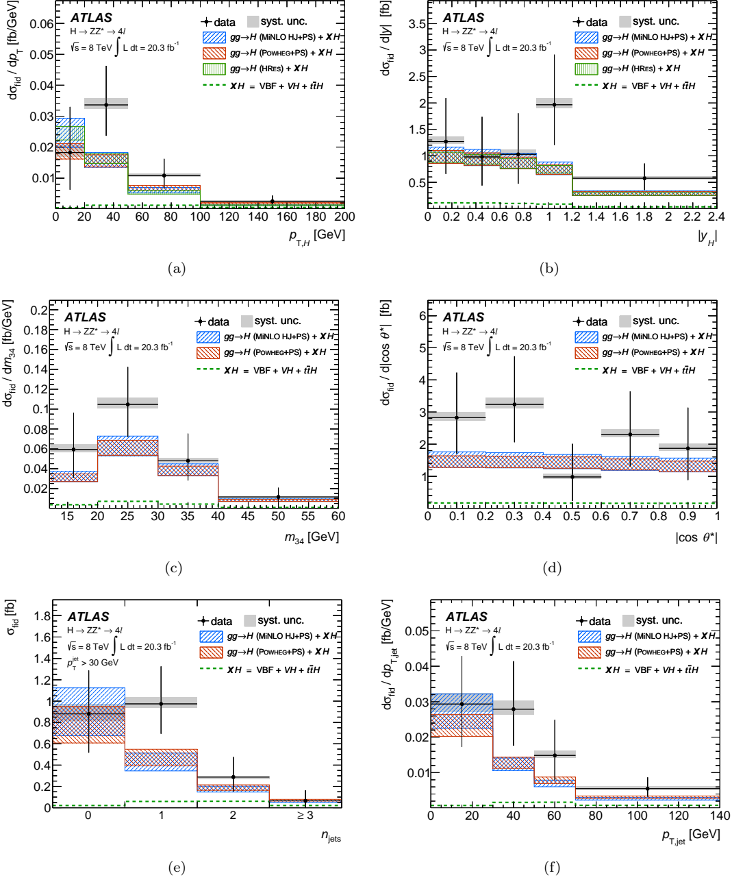
Fig. 2: Differential unfolded cross sections for the transverse momentum p_{T,H} and rapidity y_H of the Higgs boson, the invariant mass of the subleading lepton pair m_{3,4} , the magnitude of the cosine of the decay angle of the leading lepton pair in the four-lepton rest frame with respect to the beam axis |\cos\theta^*| , the number of jets n_{\text{jets}} , and the transverse momentum of the leading jet p_{T,\text{jet}} in the H \rightarrow ZZ^* \rightarrow 4l decay channel compared to different theoretical calculations of the ggF process: POWHEG, MINLO and HRES2. The contributions from VBF, ZH/WH and t\bar{t}H are determined as described in Section 2 and added to the ggF distributions. All theoretical calculations are normalized to the most precise SM inclusive cross-section predictions currently available [60]. The error bars on the data points show the total (stat. \oplus syst.) uncertainty, while the grey bands denote the systematic uncertainties. The bands of the theoretical prediction indicate the total uncertainty.
