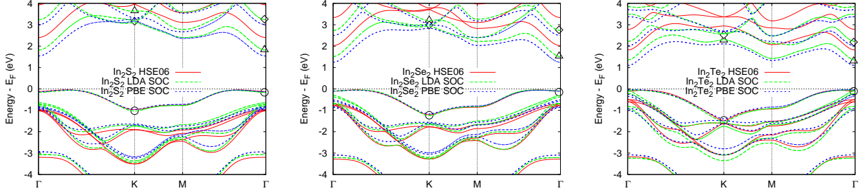
FIG. 6. (Color online) HSE06, LDA and PBE DFT band structures for \beta - \text{In}_2\text{S}_2 , \beta - \text{In}_2\text{Se}_2 , and \beta - \text{In}_2\text{Te}_2 . Spin-orbit coupling is taken into account in the case of LDA and PBE. The zero of energy is taken to be the Fermi level E_F and the bottom of the conduction band is marked with a horizontal line. The orbital composition of the \beta - \text{In}_2\text{X}_2 states highlighted by \circ , \triangle , and \diamond are summarized in the table below. Dominant contributions were found to originate from s - and p -type orbitals; the “+” and “-” subscripts refer to even (+) and odd (-) states with respect to three-dimensional inversion. The notation “ p_x p_y ” refers to equal p_x and p_y contributions as a consequence of symmetry.
