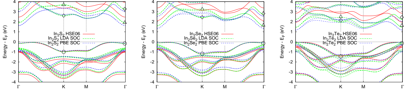
FIG. 3. (Color online) HSE06 band structures (solid red lines) for \alpha - \text{In}_2\text{S}_2 , \alpha - \text{In}_2\text{Se}_2 , and \alpha - \text{In}_2\text{Te}_2 (top panel). Spin-orbit coupling (SOC) is not included in these results. The zero of energy is taken to be the Fermi level E_F and the bottom of the conduction band is marked with a horizontal line. For comparison, the semilocal band structures are also shown, including the effects of SOC. The orbital composition of the \alpha - \text{In}_2\text{X}_2 states highlighted by \circ , \triangle , and \diamond are summarized in the table below. Dominant contributions were found to originate from s - and p -type orbitals; the “+” and “-” subscripts refer to even (+) and odd (-) states with respect to z \rightarrow -z reflection. The LDA spin-orbit splittings |\Delta E_{\text{SO}}^{\text{K}}| of the bands at the K point are also given. The notation “ p_x p_y ” refers to equal p_x and p_y contributions as a consequence of symmetry.
