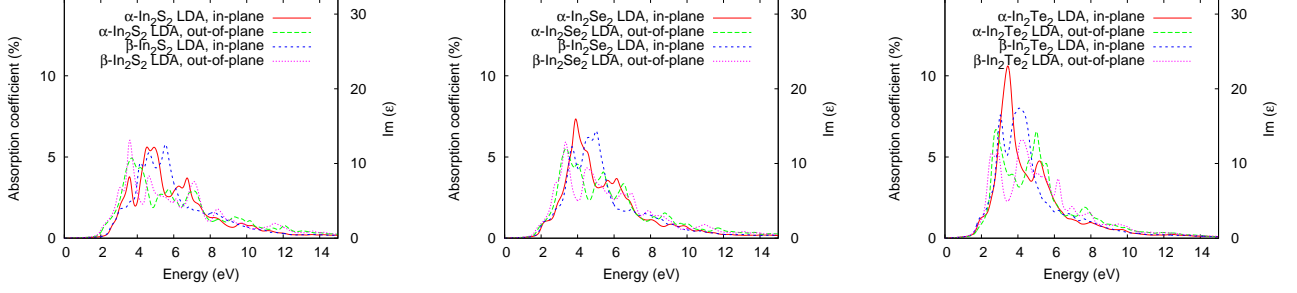
FIG. 5. (Color online) Absorption coefficient of \alpha - and \beta - \text{In}_2\text{X}_2 2D crystals as obtained from the imaginary part of the dielectric function \varepsilon by normalizing it to absolute units after it was compared to \text{Im}(\varepsilon) evaluated for graphene in the range 0.8–1.5 eV, where monolayer graphene absorbs 2.3% of light. The raw results for \text{Im}(\varepsilon) are indicated on the right-hand axis.
