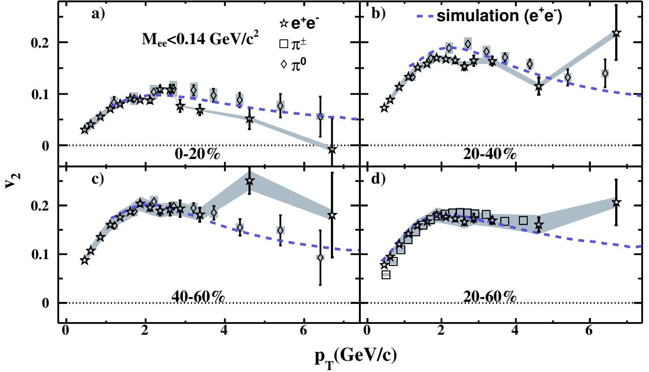
FIG. 19. (Color online) The dielectron v_2 in the \pi^0 Dalitz decay region (star symbol) as a function of p_T in different centralities from Au+Au collisions at \sqrt{s_{NN}} = 200 GeV. Also shown are the charged (square) [51], neutral (diamond) [42] pion v_2 , and the expected dielectron v_2 (dashed curve) from \pi^0 Dalitz decay. The bars and bands represent statistical and systematic uncertainties, respectively.
