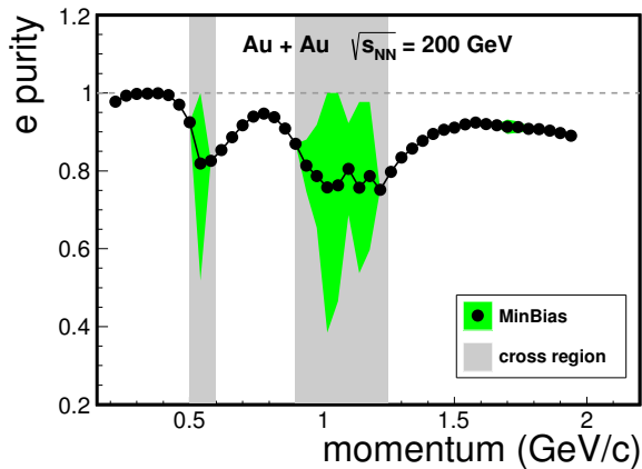
FIG. 2. (Color online) The purity of electron candidates as a function of momentum in minimum-bias Au+Au collisions at \sqrt{s_{NN}} = 200 GeV. In the cross regions, the electron candidates overlap with hadron components in the dE/dx distribution, which results in large uncertainties in the multi-component fit, as shown by the shading around the data points.
