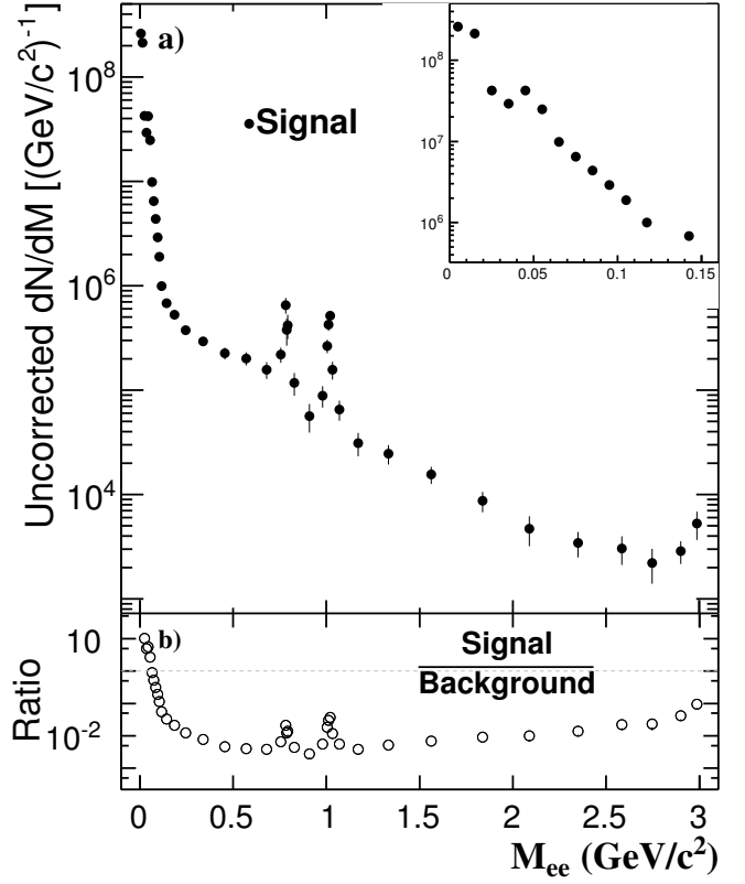
FIG. 12. Panel (a): The dielectron continuum without efficiency correction in \sqrt{s_{NN}} = 200 GeV minimum-bias Au+Au collisions. The two-peak structure, as shown in the insert, for M_{ee} < 0.12 \text{GeV}/c^2 is due to photon conversions in the beam pipe and supporting structure. Errors are statistical only. Panel (b): The signal over background ratio in \sqrt{s_{NN}} = 200 GeV minimum-bias Au+Au collisions. The first two data points are not shown for clarity. Errors are statistical.
