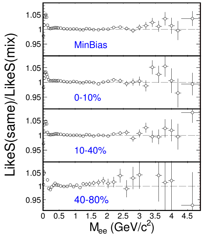
FIG. 9. (Color online) The centrality dependence of the ratio of the same-event like-sign distribution to the normalized mixed-event like-sign distribution in minimum-bias Au+Au collisions at \sqrt{s_{NN}} = 200 GeV.
