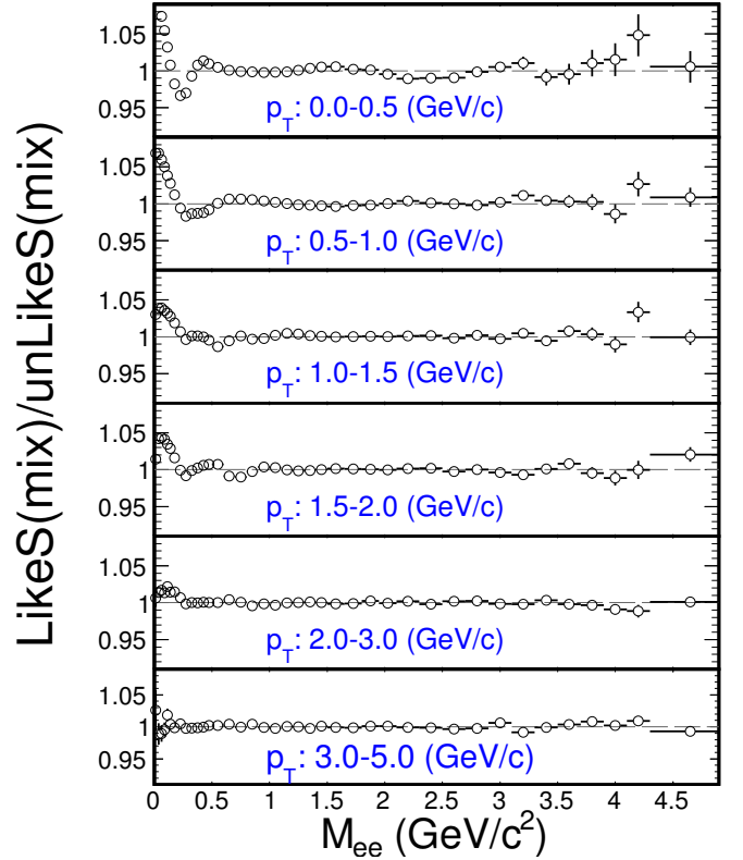
FIG. 5. (Color online) The ratio of the mixed-event like-sign distribution to the mixed-event unlike-sign distribution in different p_T ranges in minimum-bias Au+Au collisions at \sqrt{s_{NN}} = 200 GeV.
