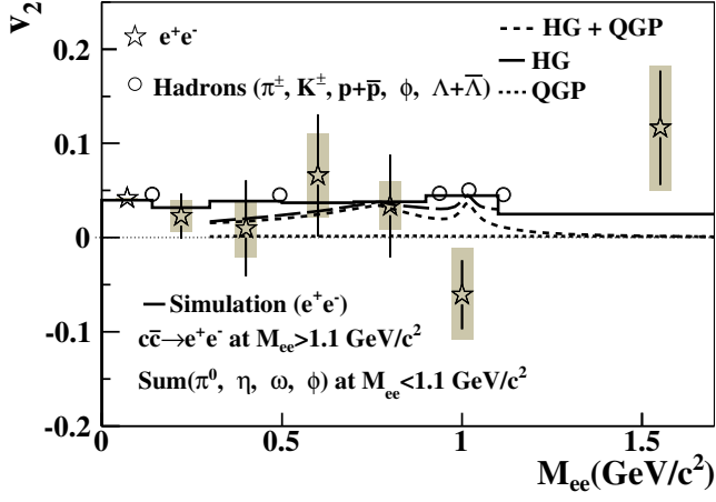
FIG. 22. (Color online) The p_T -integrated dielectron v_2 as a function of M_{ee} in minimum-bias Au+Au collisions at \sqrt{s_{NN}} = 200 GeV. Also shown are the corresponding dielectron v_2 simulated from \pi^0, \eta, \omega and \phi decays and a c\bar{c} contribution. The theoretical calculations from hadronic matter and QGP thermal radiation and the sum of these two sources [54] are shown for comparisons. The v_2 for hadrons \pi, K, p, \phi, and \Lambda are also shown for comparison. The bars and boxes represent statistical and systematic uncertainties, respectively. The systematic uncertainty for the first data point is smaller than the size of the marker.
