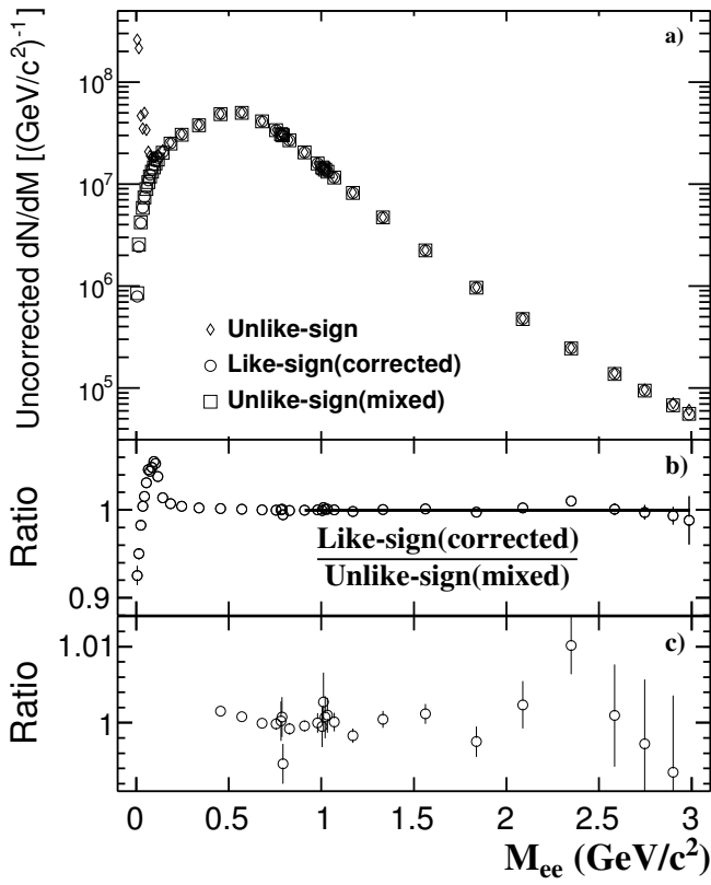
FIG. 6. (Color online) Panel (a): The electron pair invariant mass distributions for same-event unlike-sign pairs, same-event like-sign, and mixed-event unlike-sign in minimum-bias Au+Au collisions at \sqrt{s_{NN}} = 200 GeV. The electron candidates are required to be in the range |\eta| < 1 and have p_T greater than 0.2 GeV/ c . The ee pairs are required to be in the rapidity range |y_{ee}| < 1 . Variable bin widths are used for the yields and signal-to-background ratios. Panel (b): The ratio of the same-event like-sign distribution (corrected for the acceptance difference) to the normalized mixed-event unlike-sign distribution in minimum-bias Au+Au collisions at \sqrt{s_{NN}} = 200 GeV. Panel (c): A zoom-in version of Panel (b).
