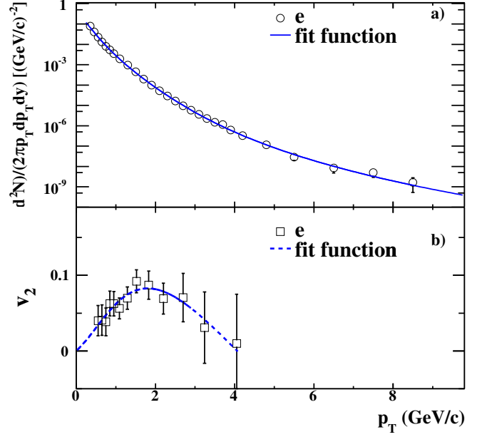
FIG. 17. (Color online) The invariant yield and v_2 of electrons from heavy flavor decays [50] fitted with functions in minimum-bias Au+Au collisions at \sqrt{s_{NN}} = 200 GeV. The spectrum is fit with a function A[e^{B\sqrt{p_T^2+C+D(p_T^2+C)} + \sqrt{p_T^2+C}/E}]^F , where A , B , C , D , E , and F are fit parameters. The v_2 is fit with the same function as used to parameterize the meson v_2 shown in Fig.15.
