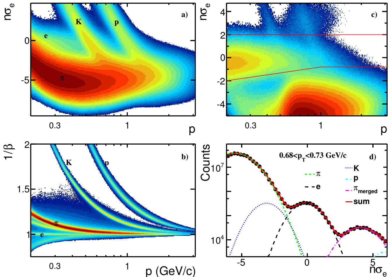
FIG. 1. (Color online) Panel (a): The normalized dE/dx distribution as a function of momentum from TPC in Au+Au collisions at \sqrt{s_{NN}} = 200 GeV. Panel (b): 1/\beta measurements from TOF versus the momentum from TPC in Au+Au collisions. The 1/\beta resolution is 0.011. Panel (c): The normalized dE/dx distribution as a function of momentum with the cut of |1/\beta - 1/\beta_{\text{exp}}| < 0.025 . An electron band is prominent with the requirement of velocity close to the speed of light from the TOF measurement. Electron candidates whose n\sigma_e falls between the lines are selected for further dielectron analysis. Panel (d): The n\sigma_e distribution for 0.68 < p_T < 0.73 GeV/c after the cut |1/\beta - 1/\beta_{\text{exp}}| < 0.025 is applied. The solid curve represents a multiple Gaussian fit to the n\sigma_e distribution. Different components from the fit are also shown. The \pi_{\text{merged}} represents contribution from two merged \pi tracks.
