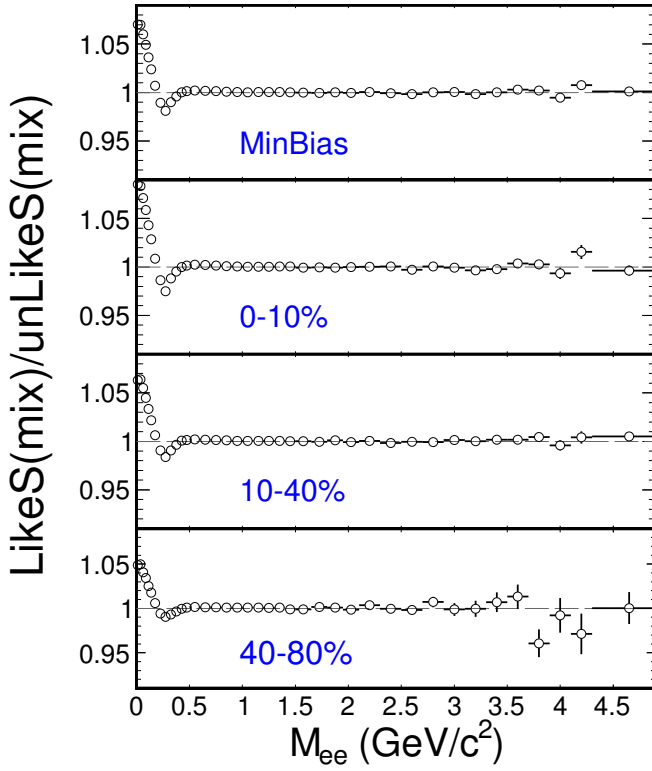
FIG. 4. (Color online) The ratio of the mixed-event like-sign distribution to the mixed-event unlike-sign distribution in minimum-bias, as well as specific centrality selections of, Au+Au collisions at \sqrt{s_{NN}} = 200 GeV.
