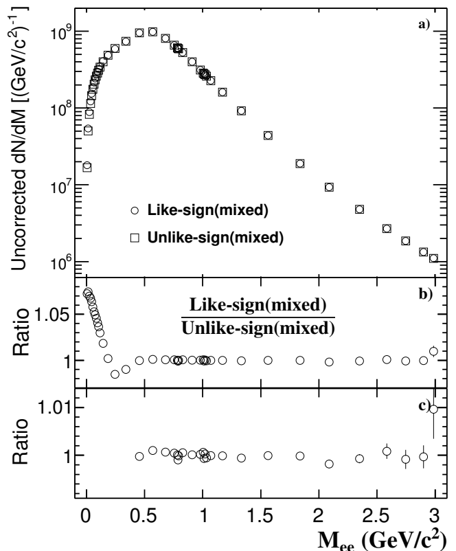
FIG. 3. (Color online) Panel (a): The mixed-event unlike-sign and mixed-event like-sign electron pair invariant mass distributions in minimum-bias Au+Au collisions at \sqrt{s_{NN}} = 200 GeV. Panel (b): The ratio of mixed-event like-sign distribution to mixed-event unlike-sign distribution in minimum-bias Au+Au collisions at \sqrt{s_{NN}} = 200 GeV. Panel (c): A zoom-in version of Panel (b).
