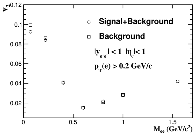
FIG. 14. The v_2 for the same-event unlike-sign electron pairs (circles) and background (squares) as a function of M_{ee} within STAR acceptance in minimum-bias Au+Au collisions at \sqrt{s_{NN}} = 200 GeV.
