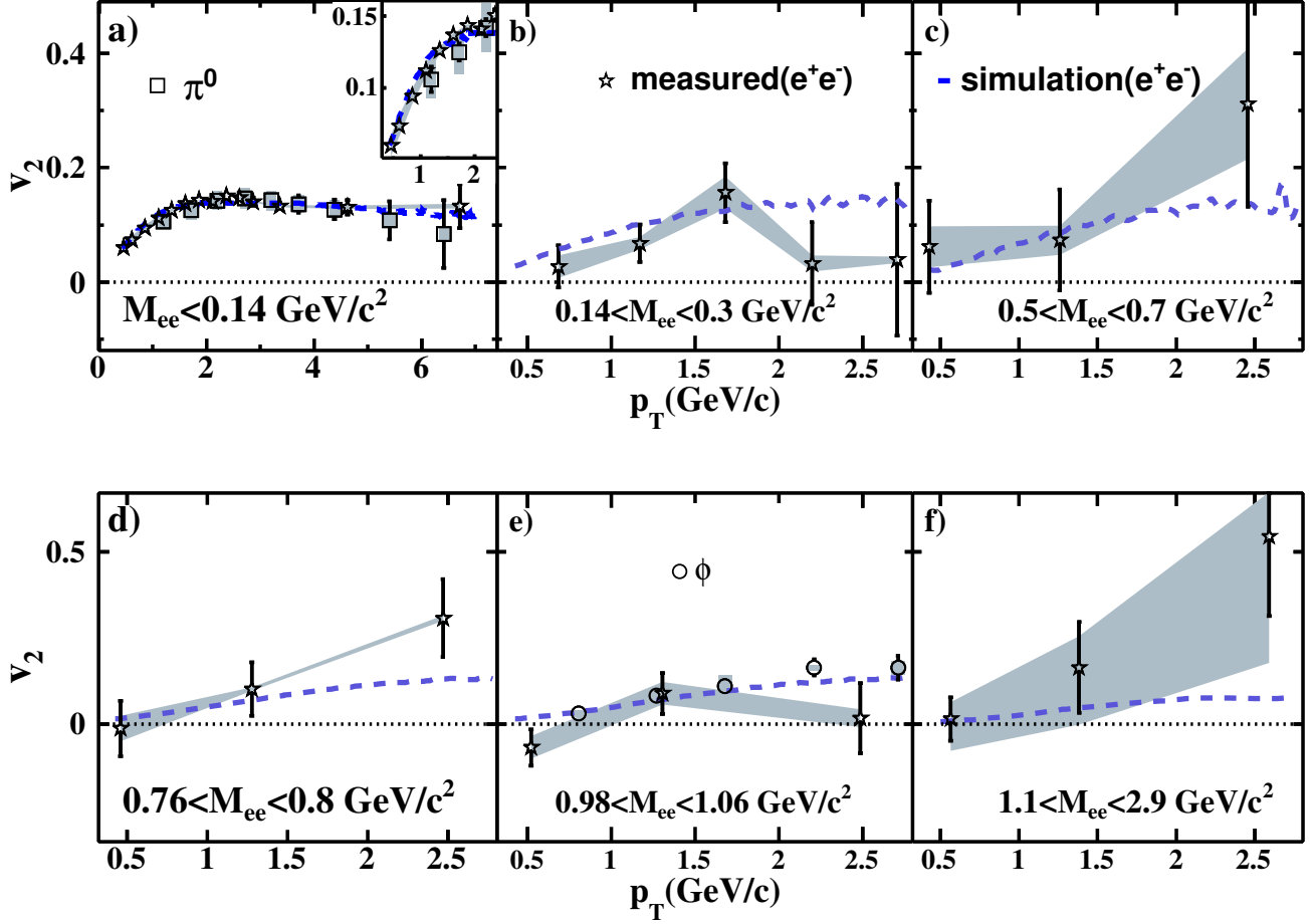
FIG. 21. (Color online) Panels (a-f): The dielectron v_2 as a function of p_T in minimum-bias Au+Au collisions at \sqrt{s_{NN}} = 200 GeV for six different mass regions: \pi^0 , \eta , charm + \rho^0 , \omega , \phi , and charm+thermal radiation. Also shown are the neutral pion [42] v_2 and the \phi meson v_2 [44] measured through the decay channel \phi \rightarrow K^+K^- . The expected dielectron v_2 (dashed curves) from \pi^0 , \eta , \omega and \phi decays in the relevant mass regions are shown in panels (a-e) while that from c\bar{c} contributions is shown in panel (f). The bars and bands represent statistical and systematic uncertainties, respectively. The full difference between mixed-event unlike-sign and same-event like-sign background subtraction contributes to the lower bound of the systematic uncertainties, which leads to asymmetric systematic uncertainties in panel (f).
