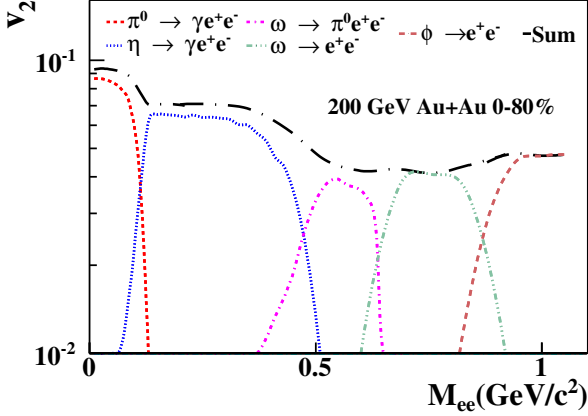
FIG. 16. (Color online) The simulated v_2 as a function of M_{ee} from \pi^0 , \eta , \omega and \phi decays within the STAR acceptance in minimum-bias Au+Au collisions at \sqrt{s_{NN}} = 200 GeV, including the contributions from specific decays. The contribution from \phi \rightarrow \eta e^+ e^- is smaller than 1% and is not shown for clarity. The bin width is 20 MeV/ c^2 .
