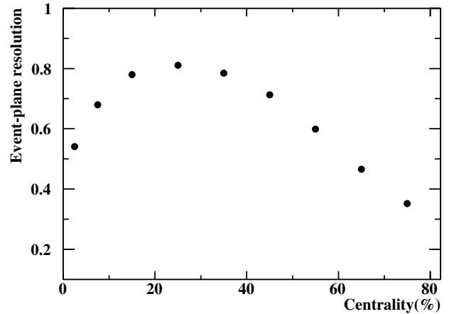
FIG. 13. The event-plane resolution from central to peripheral (left to right) collisions in minimum-bias Au+Au collisions at \sqrt{s_{NN}} = 200 GeV.
