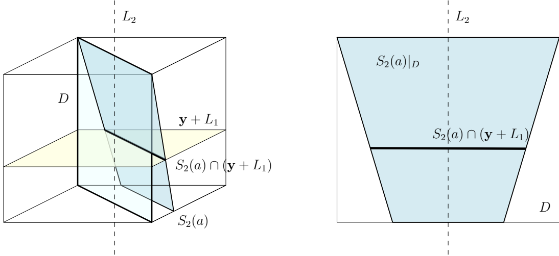
FIGURE 3. Sections of S_2(a) and \mathbf{y} + L_1 in Q_{n-1} and its diagonal section D .
