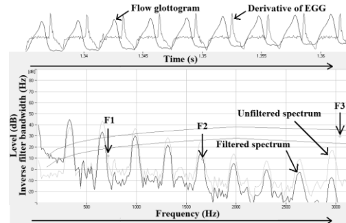
Figure 2: Inverse filtering with DeCap (after Sundberg et al. 2013). The upper panel shows the inverse filtered signal and the dEGG (dark and light colors, respectively); the lower panel shows the audio spectrum, and the spectrum of the filtered flow (light and dark colors, respectively). The arrows with the labels F1, F2, F3 show the first three formants adjusted for inverse filtering.
