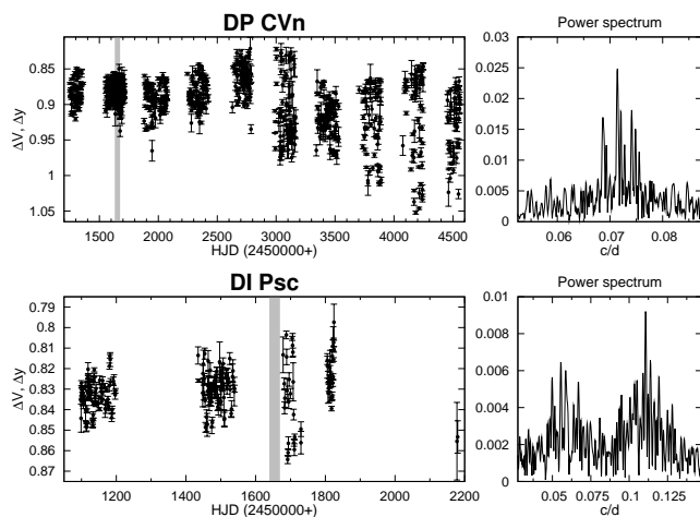
Fig. 2. \Delta V and \Delta y magnitudes and periodograms from the APT data of DP CVn (top) and DI Psc (bottom). The vertical grey stripes indicate the time of our Doppler imaging data. The photometric periods adopted for this work are 14.010 d (DP CVn) and 18.066 d (DI Psc, but see also Sect. 3.2 for details).
