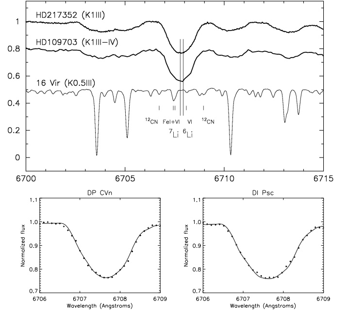
Fig. 4. Top panel: Li I 6708 Å spectra of DI Psc (top) and DP CVn (shifted by -0.2). Also shown is a spectrum of the inactive K0.5III giant 16 Vir (shifted to bottom) for comparison purpose. The measured equivalent width of the lithium line of DI Psc and DP CVn is 328±5 mÅ and 316±7 mÅ, respectively. Bottom panels: Li I 6708 Å line fitted by synthetic spectra for DP CVn (left) and DI Psc (right), resulting in logarithmic abundances of \log n(\text{Li})=2.28 , and of 2.20, respectively.
