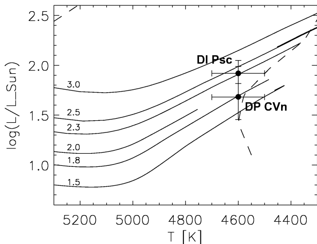
Fig. 1. The observed positions of DP CVn and DI Psc in the Hertzsprung-Russell diagram. The post-main-sequence tracks for 1.5, 1.8, 2.0, 2.3, 2.5 and 3.0 solar masses are shown (c.f. Granzer et al. 2000). These tracks suggest masses of 1.8 M_{\odot} and 2.3 M_{\odot} for DP CVn and DI Psc, respectively. Both stars appear on the RGB at the end of the first Li dredge-up phase, which is marked by the dashed lines taken from Charbonnel & Balachandran (2000).
