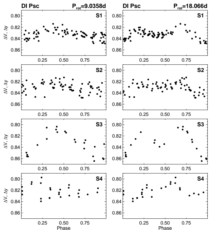
Fig. 3. Folded light curves of DI Psc for four observing runs between HJD 2451098.7 and HJD 2451825.8 (S1-S4 from top to bottom panels, respectively), assuming rotation period of either 9.0358 d (left panels) or 18.066 d (right panels), according to the power spectrum in Fig. 2 bottom. Note that using 18.066 d yields less scattered light curves. For a quantitative comparison see Sect. 3.2.
