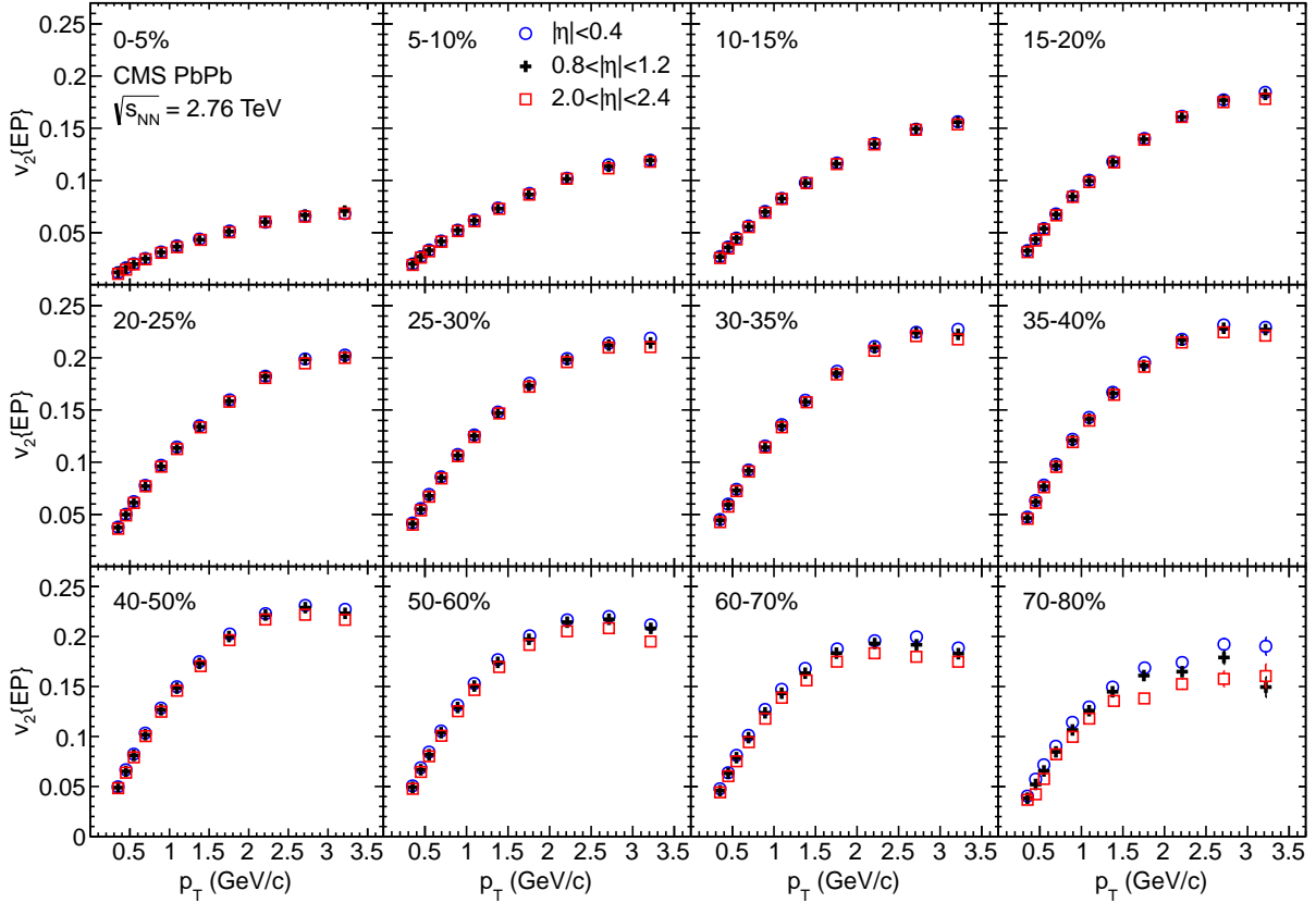
Figure 14: (Color online) Results from the event-plane method for v_2(p_T) in three pseudorapidity regions and in 12 centrality classes. The error bars show the statistical uncertainties that in most cases have magnitudes smaller than the size of the symbol.
