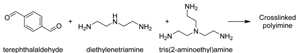
Fig. 1. Synthesis of the crosslinked polyimine (based on [13]).
