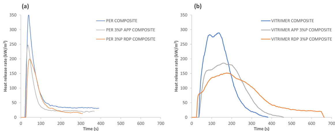
Fig. 6. The heat release rate of heat release rate of reference and flame retarded (a) epoxy resin and (b) vitrimer composites.
