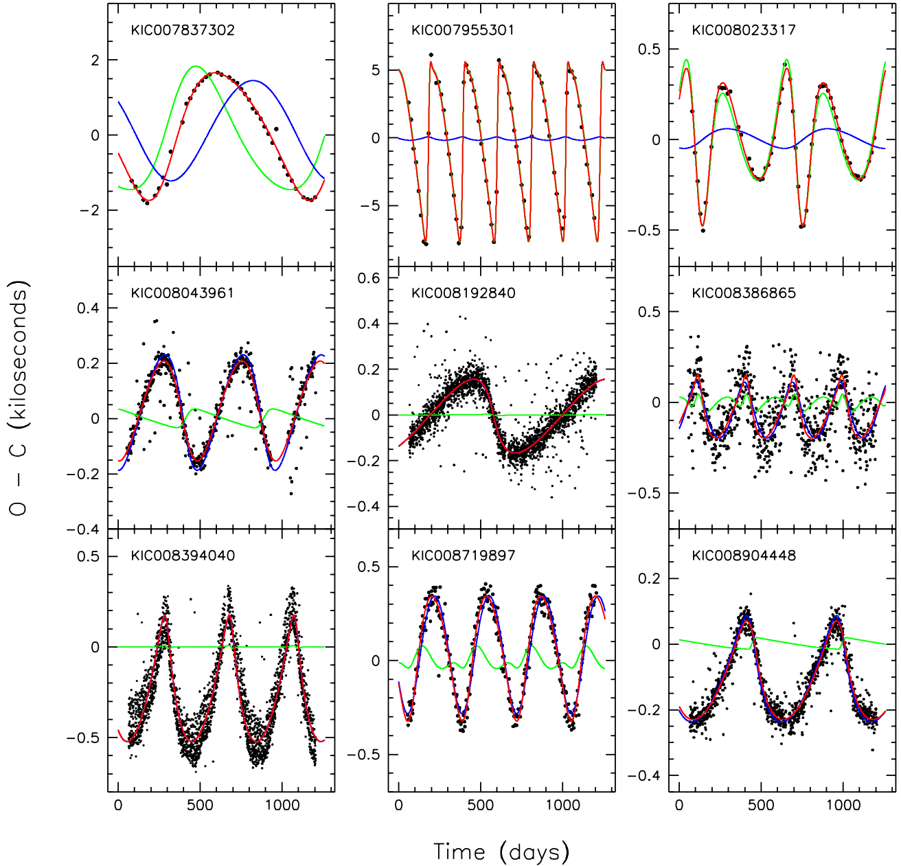
Figure 3. O-C data and model fits for 9 systems with KIC numbers between 7837302 and 8904448. The red curves are the total model O-C values. Dark blue is the model fit for the Roemer delay (eq. (6)). Light green curves represent the total physical delay (sum of eqs. (8) and (9)). Note that the vertical scales are different on all of the plots; the amplitudes of the O-C curves range from a low of \sim 150 sec to a high of 6000 sec. The linear and quadratic terms in the fit have been subtracted before the plot is made.
