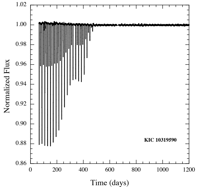
Figure 10. Example of a system (KIC 10319590) where the eclipse depths exhibit strong variations with time. In this extreme case, the eclipses completely disappear after \sim 400 days, presumably due to the precession of the binary orbital plane caused by the presence of the inferred third body.
