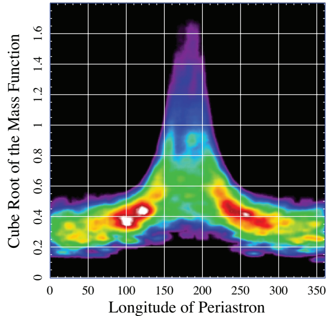
Figure 9. Example of the correlation between the cube root of the mass function, f(M_3)^{1/3} , and the longitude of periastron, \omega , of the orbit of the triple for a system in which the physical and Roemer delays are comparable: KIC 9451096. The colors are scaled according to the relative probability with white and red the highest, blue and purple the lowest.
