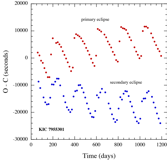
Figure 11. Example of a system (KIC 7955301) where the O-C curves for the primary and secondary eclipses lie on “divergent” paths – at least for the 3-year duration of the Q1-Q13 data. As well, the two O-C curves even have somewhat different profiles.
