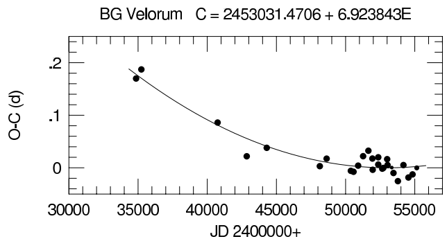
Figure 10. O–C diagram of BG Vel. The plot can be approximated by a parabola indicating a continuously increasing pulsation period.
