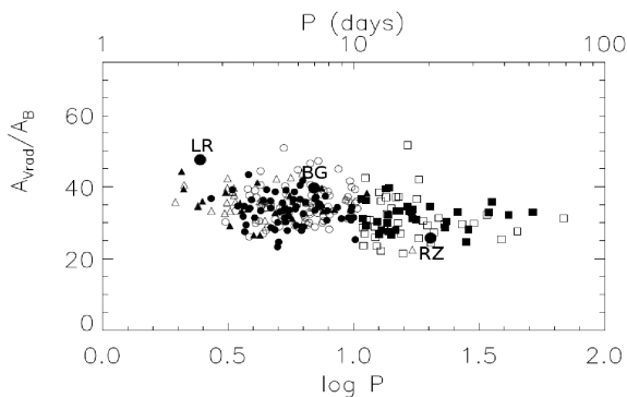
Figure 14. The slightly excessive value of the A_{V_{\text{RAD}}}/A_B amplitude ratio of LR TrA and BG Vel (large circles) with respect to the average value characteristic at the given pulsation period is an independent indication of the presence of a companion star. This is a modified version of fig. 4f of Klagyivik & Szabados (2009). The open symbols in the original figure correspond to known binaries and the filled symbols to Cepheids without known binary. For the meaning of various symbols, see Klagyivik & Szabados (2009).
