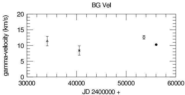
Figure 13. \gamma -velocities of BG Vel. The symbols for the different data sets are the same as in Fig. 12.
