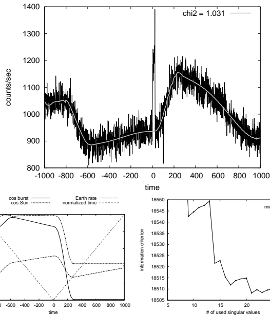
Fig. 25. Top: Lightcurve of the Fermi GRB 100414.097 as measured by the non-triggered GBM detector '5' and the fitted background with a grey line. Burst interval: [-20:30]. Bottom left: Underlying variables (absolute values). See Sec. 3. Bottom right: Akaike Information Criterion. See Sec. 4.4.
