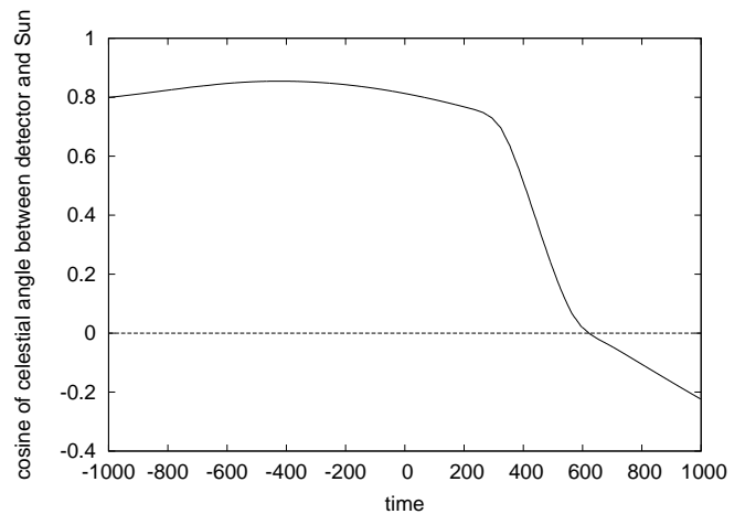
Fig. 6. The celestial distance of the 3rd GBM detector and the Sun as a function of time during the GRB 091030.613. The dashed line shows the 0 level (under this the Sun and the detector close in an angle larger than 90^\circ ). It is worth comparing this figure to Fig. 1.
