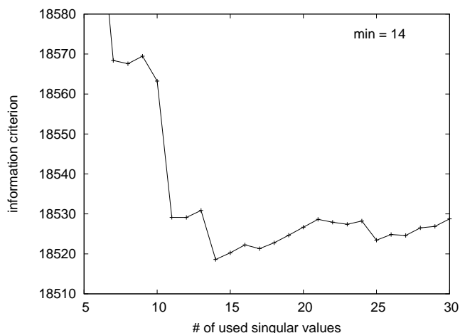
Fig. 8. The Akaike Information Criterion for model selection. Model with 14 singular values is selected. (First and last five singular values are usually too high, so we do not show them.)
