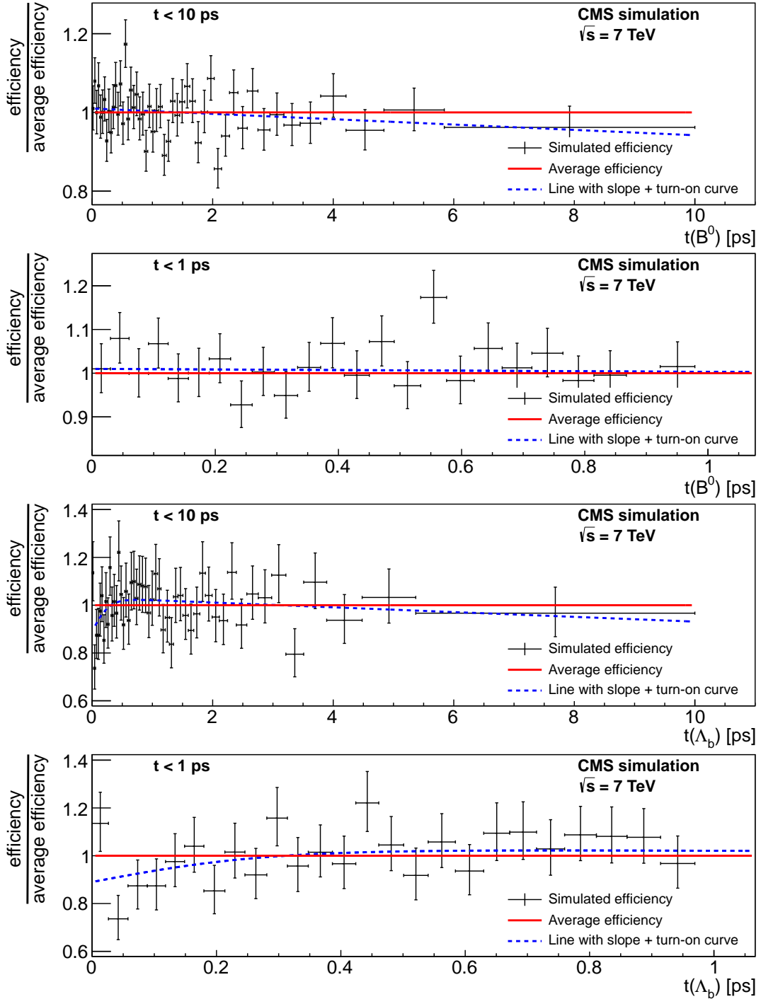
Figure 1: The ratio of the reconstruction and selection efficiencies to the overall average efficiency as a function of proper decay time for B^0 (upper two plots) and \Lambda_b^0 (lower two plots). The second and fourth plots show the B^0 and \Lambda_b^0 efficiency ratios, respectively, for smaller proper decay times t < 1 ps. The horizontal solid lines show a ratio of 1, while the dashed lines display the results from fitting the efficiencies to the function given by Eq. (2).
