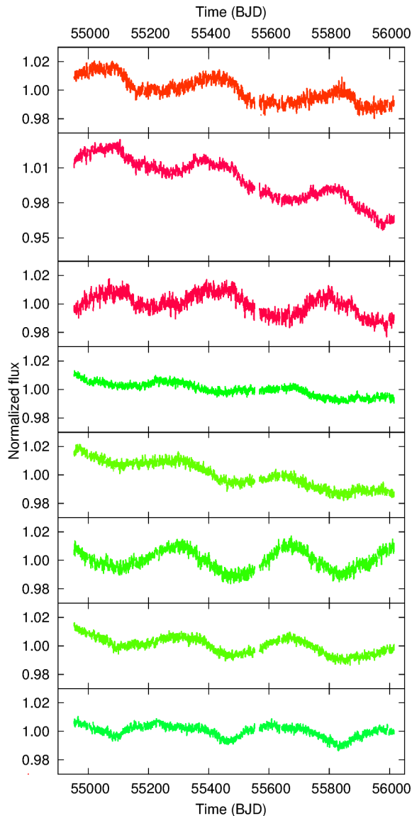
Figure 5. Examples of light curves showing variability with a period equal a Kepler -year. Colours are indicating groups of stars with different phase of the Kepler -year. Note the apparent alternation of the red (top three) and green (bottom five) light curves. (See the electronic version of the article for the figure in colours.)
