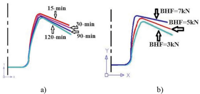
Fig. 10. a) Effect of transfer time at 5 kN, b) effect of BHF at 15-min edging time
