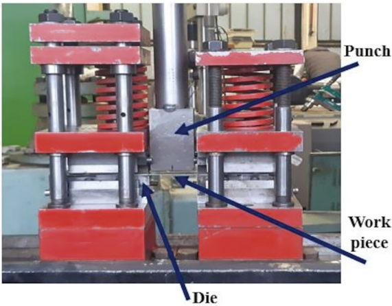
Fig. 7. U-draw bending die apparatus
