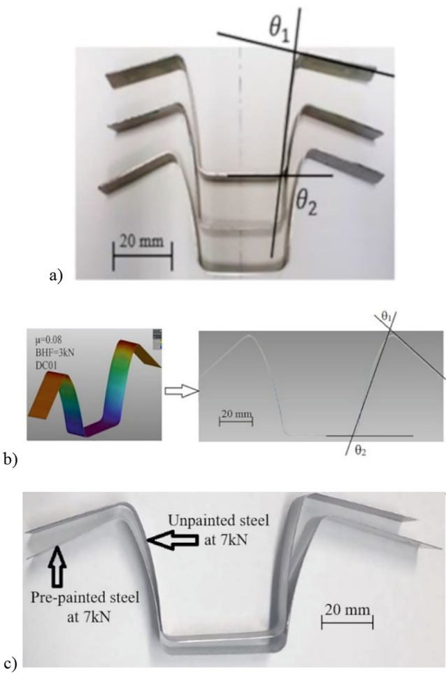
Fig. 8. NUMISHEET '93 benchmark standard for springback prediction [19], a) WT AA6082 at 15-min transfer time, b) unpainted steel at 3 kN BHF, c) the difference of springback for unpainted and pre-painted steel at 7 kN BHF
