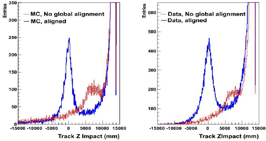
Fig. 18. Track Z_{Impact} parameters (see section 4.1.1 for its definition) reconstructed in one of the T2 quarter (left plot from simulation and right from data). The blue (red) curve is obtained with (without) the inclusion of the global alignment corrections.
