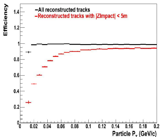
Fig. 20. Efficiency of single pion reconstruction as a function of the particle p_T . The red and black curves show respectively the p_T acceptance obtained with and without applying the primary selection cut on the Z_{Impact} parameter.
