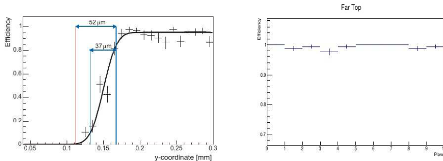
Fig. 2. Left plot: particle detection efficiency for a TOTEM silicon detector as a function of the distance ( y ) from its mechanical edge. Right plot: hit efficiency of the 10 detectors of one pot for one of the \beta^* = 90 m run (statistics: 2500 tracks).
