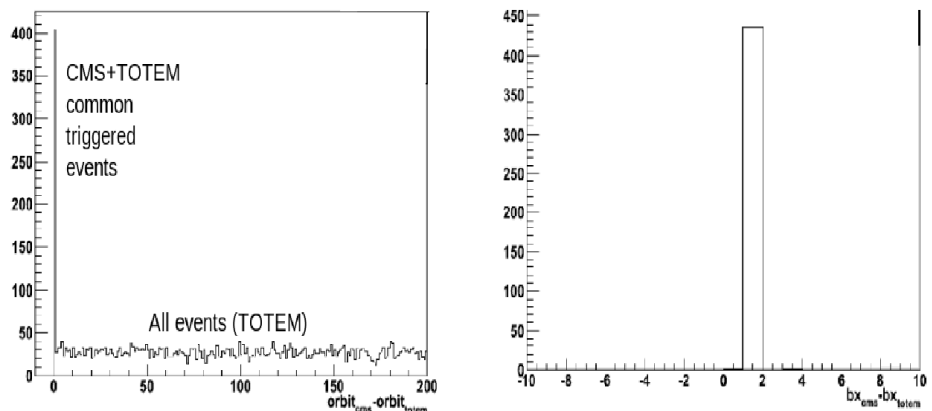
Fig. 29. Distribution of offset of the orbit number (left) and of the bunch number (right) for a reconstructed run.
