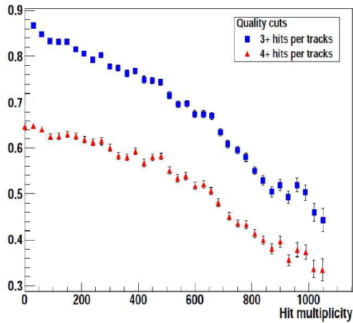
Fig. 23. The simulated efficiency of primary tracks reconstruction: the red triangle points have an added quality requirement of 4 points per track, while the blue square ones define a track only with three points (see text).
