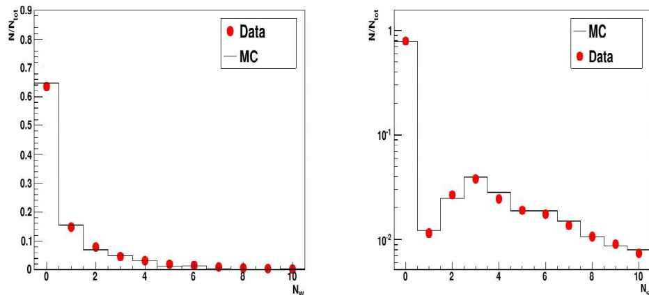
Fig. 21. Comparison between MC and data for the T1 CSC detector simulation, left plot shows the number of anode wires with signal per each event, right plot the same for the cathode strips.
