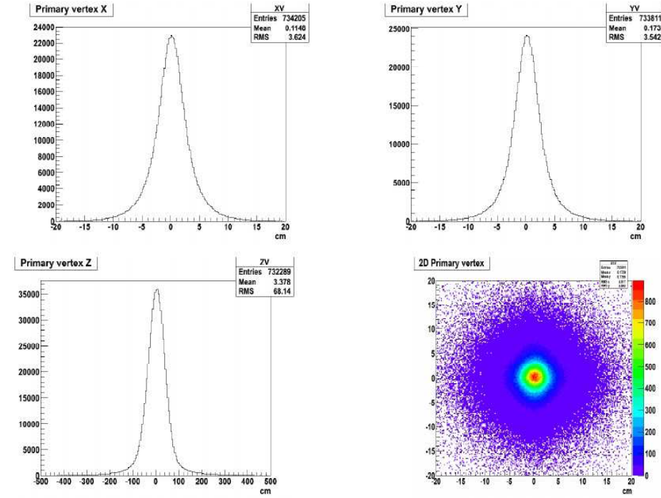
Fig. 26. Vertex position distribution as reconstructed with the T1 data.
