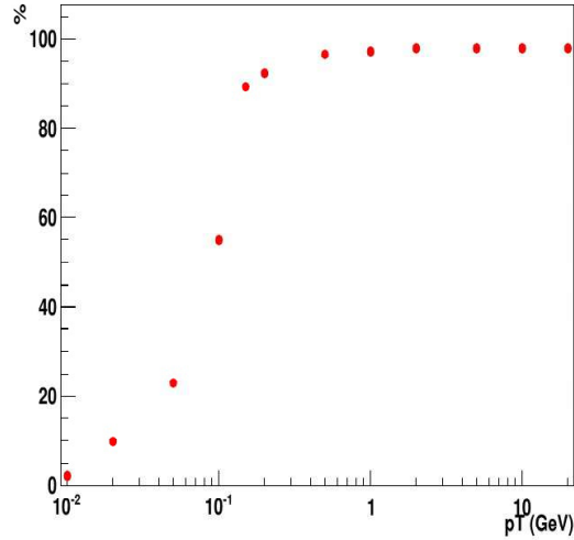
Fig. 22. The p_T acceptance of the T1 telescope.
