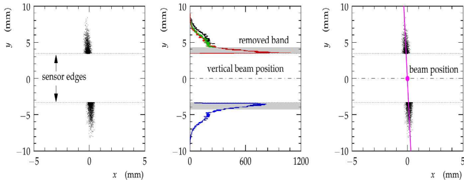
Fig. 9. Alignment with selected elastic events. Left plot: a selection of elastic events; center plot: vertical alignment; right plot: horizontal alignment and the unit rotation are established by fitting the track distribution. The procedure is discussed in detail in the text.
