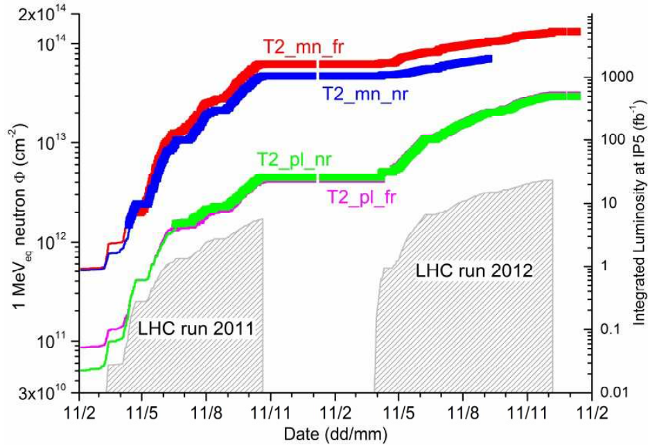
Fig. 30. Cumulated 1 MeV-neutron equivalent fluence measured with the p-i-n diode sensors: CMRP in the low fluence range (continuous lines), and BPW in the high-fluence range (square markers) for the TOTEM T2 Telescope during the first 3 years of LHC runs. The evolution of the integrated luminosity delivered in IP5 during 2011 and 2012 is added for comparison (the gray hashed region).
