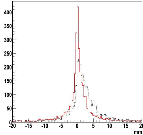
Fig. 25. Residuals for the T1 detectors before and after the alignment procedure: the black dotted line is the distribution of the values before, the red continuous line after the alignment operation.
