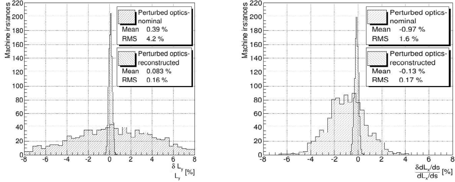
Fig. 6. Relative error distribution of L_y for beam 1 before and after matching (left) and of dL_x/ds for beam 1 before and after matching(right).
