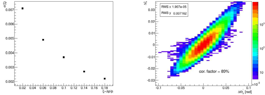
Fig. 13. Left plot: momentum reconstruction resolution for a diffractive protons sample. Right plot: correlation between the errors in \Theta_x^* and \xi .
