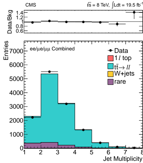
Figure 5: Comparison of the jet multiplicity distributions in data and MC simulation in the sample dominated by t\bar{t} \rightarrow ll events.
