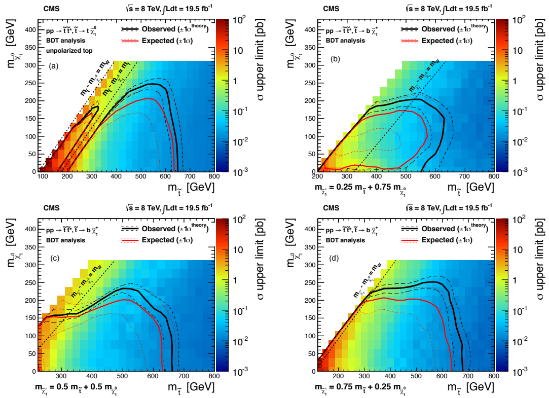
Figure 10: Interpretations using the primary results from the BDT method. (a) \tilde{t} \rightarrow t\tilde{\chi}_1^0 model; (b) \tilde{t} \rightarrow b\tilde{\chi}_1^+ model with x = 0.25 ; (c) \tilde{t} \rightarrow b\tilde{\chi}_1^+ model with x = 0.50 ; (d) \tilde{t} \rightarrow b\tilde{\chi}_1^+ model with x = 0.75 ; The color scale indicates the observed cross section upper limit. The observed, median expected, and \pm 1\sigma expected 95% CL exclusion contours are indicated. The variations in the excluded region due to \pm 1\sigma uncertainty of the theoretical prediction of the cross section for top-squark pair production are also indicated.
