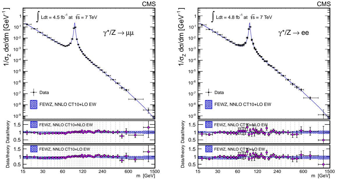
Figure 4: The DY dimuon and dielectron invariant-mass spectra normalized to the Z-boson production cross section ( 1/\sigma_Z d\sigma/dm ), as measured and as predicted by FEWZ+CT10 NNLO calculations, for the full phase space. The vertical error bars for the measurement indicate the experimental (statistical and systematic) uncertainties summed in quadrature with the theoretical uncertainty resulting from the model-dependent kinematic distributions inside each bin. The shaded uncertainty band for the theoretical calculation includes the statistical uncertainty from the FEWZ calculation and the 68% confidence level uncertainty from PDFs combined in quadrature. The effect of NLO EW correction including \gamma\gamma -initiated processes (LO EW correction only) is shown in the middle (bottom) plot for each channel. The data point abscissas are computed according to Eq. (6) in Ref. [48].
