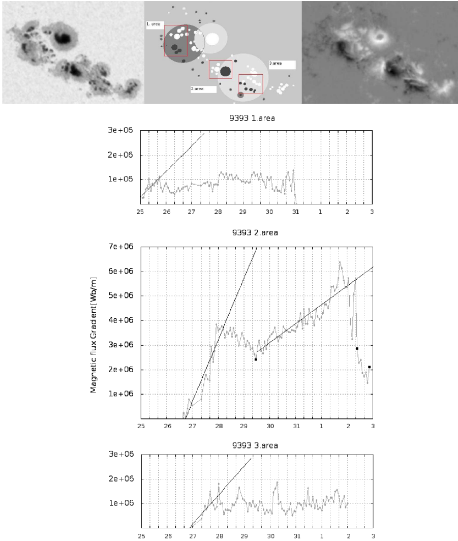
Figure 3: Upper panel: White-light view of the NOAA 9393 active region on 29 March 2001 (left panel), its magnetogram (right panel) and the schematic view of the sunspot group reconstructed from the SDD (middle panel), the umbrae are represented by circles of corresponding area, the polarities are shown by colors. Lower panel: Variation of the horizontal magnetic flux gradient in the three boxes indicated in Figure 3 between 25 March and 3 April, 2001. Black squares show the times of flares.
