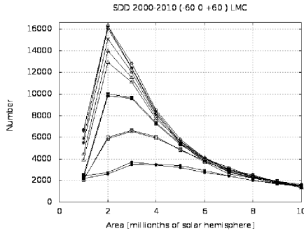
Figure 2: Dependence of the numbers of umbrae on their sizes and positions. The symbols mean longitudinal bins measured from the central meridian in degrees: open circles: 0-10, stars: 10-20, triangles: 20-30, black squares: 30-40, open squares: 40-50, black dots: 50-60. The double curves refer to the eastern and western halves of the disc, they are practically identical.
