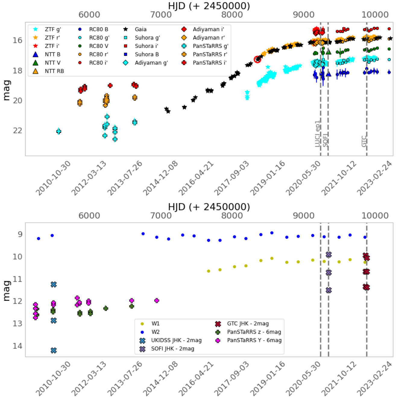
Fig. 2. Visible (top) and IR (bottom) light curves of Gaia18cjb. The red circle highlights the Gaia Alert trigger. The error bars smaller than the symbol size are not presented. Grey dashed lines correspond to the epochs for which we collected NIR spectroscopy.
