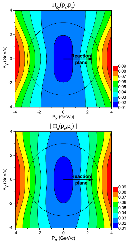
FIG. 3. (Color online) The dominant y -component and the modulus of the observable polarization, \Pi_0(\mathbf{p}) in the rest frame of the emitted \Lambda as a function of the \Lambda momentum in the transverse plane at the participant c.m. (i.e. at p_z = 0 ).
