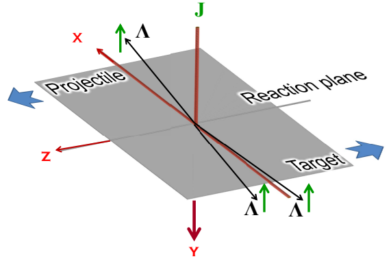
FIG. 1. (Color online) Sketch of a peripheral heavy ion collisions at high energy. The \Lambda polarization points essentially into the direction of the total angular momentum ( -y ) of the interaction region, orthogonal to the reaction plane. \Lambda s with the largest polarization are emitted into the (xz) reaction plane.
