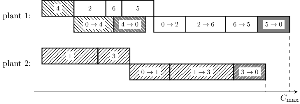
Figure 5: Example for a solution for the IPODS-MP with 2 plants. Orders 2, 4, 5, and 6 are assigned to the first, orders 1 and 3 are assigned to the second plant.
