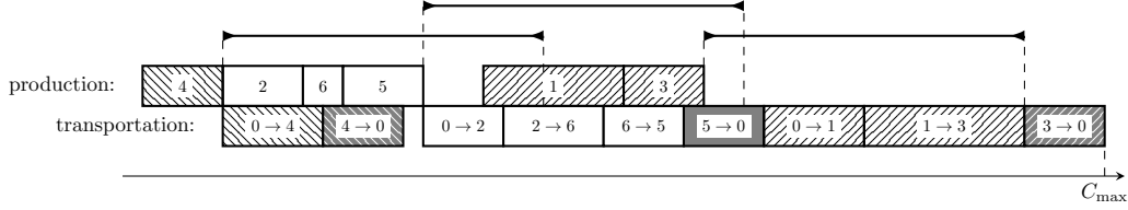
Figure 1: Example for a solution. Six orders are grouped into three batches depicted with different patterns. Lifespan intervals are depicted above the GANTT chart.
