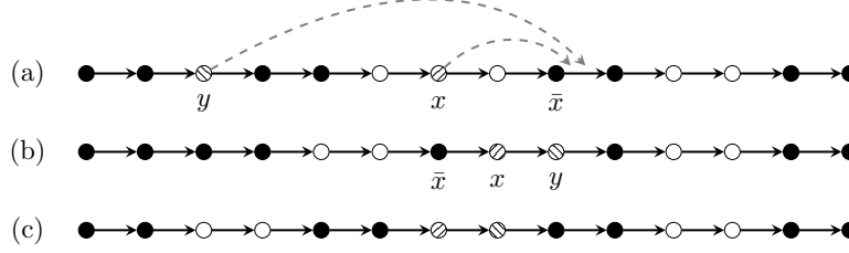
Figure 4: Example for a double relocation. (a) Initial solution. (b) Solution after change. (c) Solution after bringing it to canonical form again.
