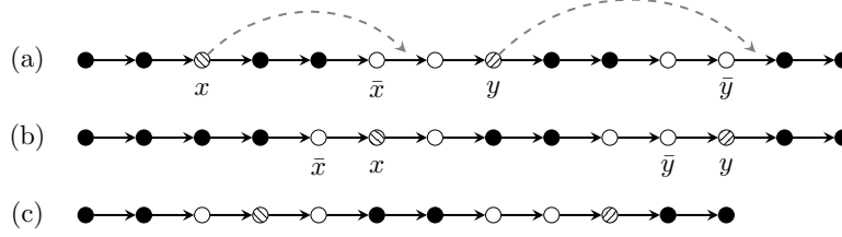
Figure 3: Example for a knockout operation. (a) Initial solution. (b) Solution after change. (c) Solution after bringing it to canonical form again.
