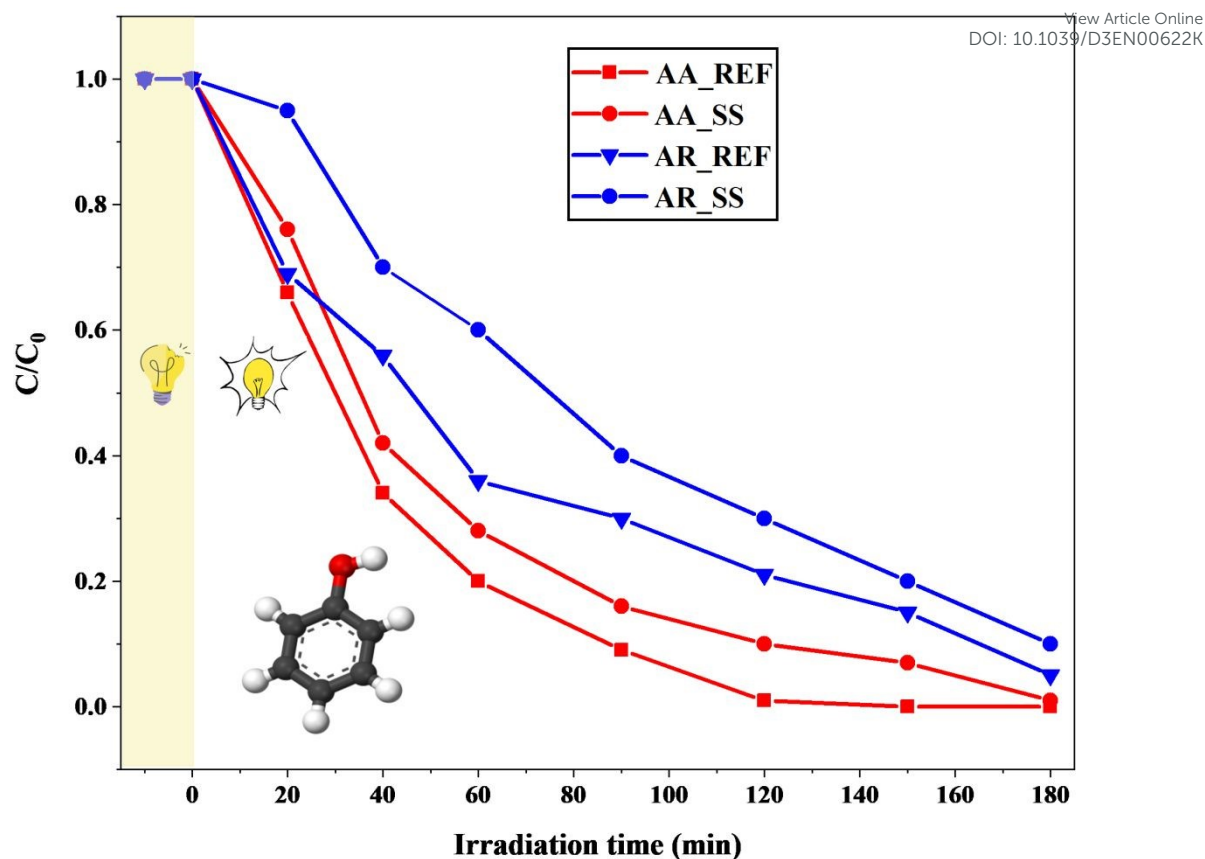
Fig. 9. Phenol degradation curves using Aldrich Anatase and Aldrich Rutile as references before and after interactions with the soil solution.
