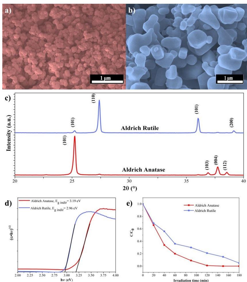
Fig. 2. Characterization of TiO 2 NPs: a) SEM-micrographs of Aldrich Anatase and b) Aldrich Rutile; c) XRD-patterns of Aldrich Anatase and Aldrich Rutile; d) band gap of Aldrich Anatase and Aldrich Rutile; e) phenol degradation performance.
