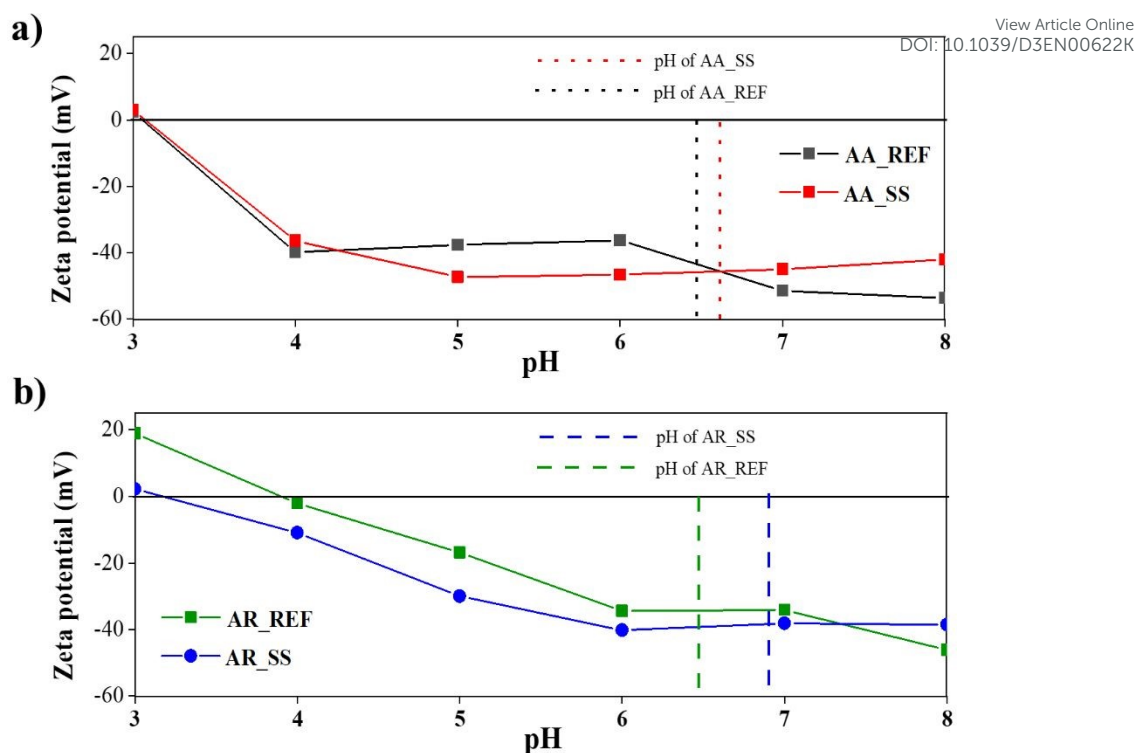
Fig. 5. ZP and IEP of TiO 2 NPs: a) AA_REF: reference Aldrich Anatase, AA_SS: Aldrich Anatase in soil solution; b) AR_REF: reference Aldrich Rutile, AR_SS: Aldrich Rutile in soil solution).
