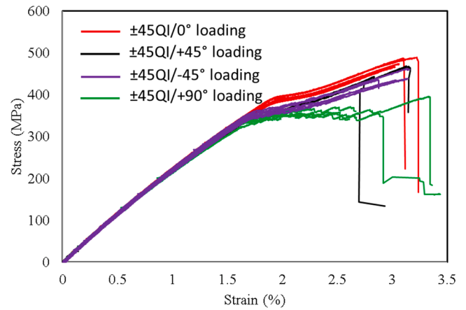
Fig. 4.10. Pseudo-ductile response of glass/carbon hybrid loaded in four fibre directions. Layup [45_{\text{S-glass}}/90_{\text{S-glass}}/-45_{\text{S-glass}}/0_{\text{S-glass}}/0_{\text{C-T300}}/45_{\text{C-T300}}/90_{\text{C-T300}}/-45_{\text{C-T300}}]_s [139].
