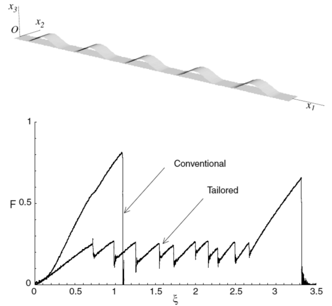
Fig. 3.9. Normalised load-displacement response of tailored undulating energy absorber concept versus conventional straight fibres [80].
