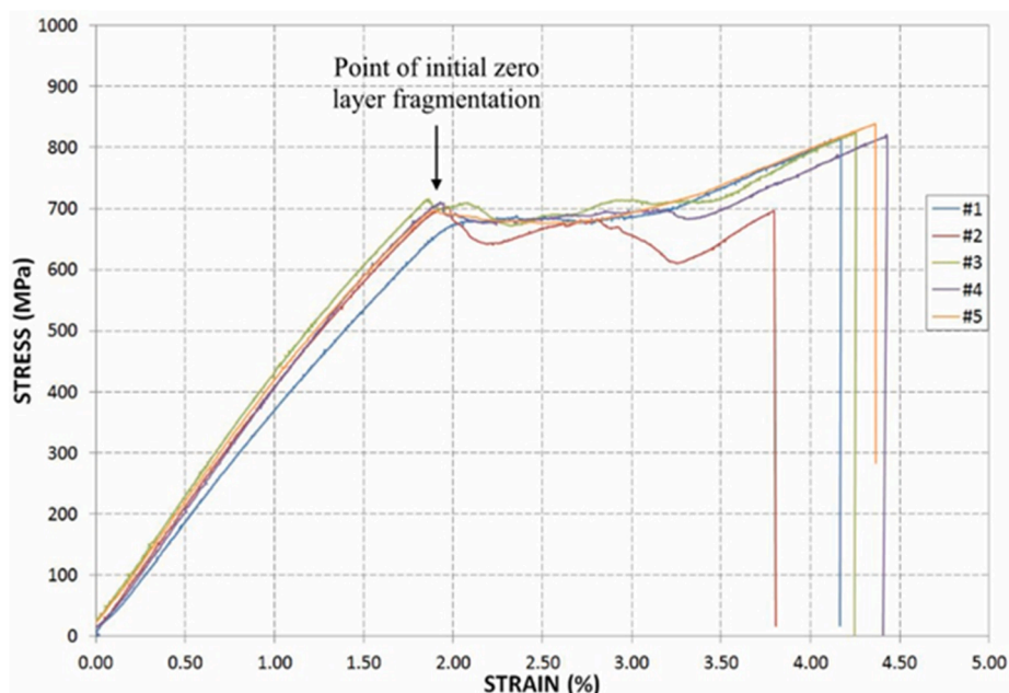
Fig. 4.16. Pseudo-ductile tensile response of [\pm 26/0]_S laminate [172].
