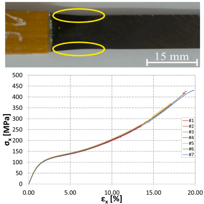
Fig. 3.2. Necking and non-linear tensile response of thin-ply \pm 45 angle-ply carbon/epoxy laminates [66].
