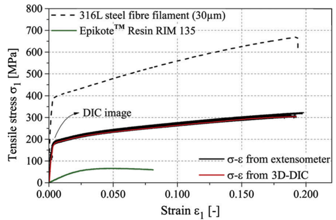
Fig. 2.15. Ductile steel/epoxy composite and its constituents [50].
