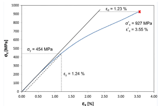
Fig. 3.4. Response of thin-ply \pm 25^\circ carbon/epoxy laminate [66].
