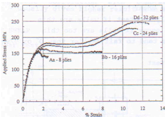
Fig. 3.1. Tensile behaviour of [(+45/-45)_n]_s carbon/epoxy laminates, n = 1, 2, 3, 4 [61].
