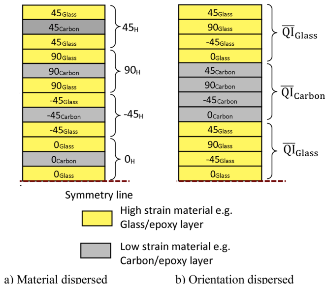
Fig. 4.9. Alternative quasi-isotropic hybrid configurations.
