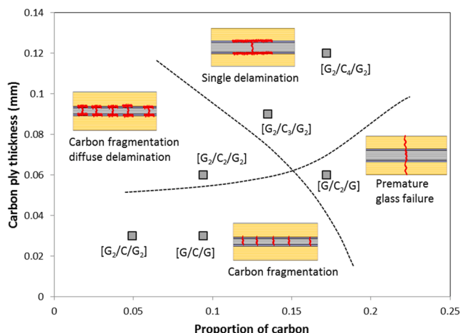
Fig. 4.5. Damage mode map for E-glass/thin carbon hybrid composite [106].
