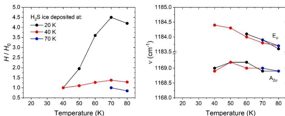
Fig. 5. Variations in peak height H (left panel) and peak positions \nu (right panel) of the \nu_2 modes for H_2S ices deposited at 20 (black circles), 40 (red circles), and 70 K (blue circles). Note that the variations in H are reported relative to their initial values H_0 upon deposition of the ice. Error bars have been omitted for clarity, but upper bounds to the uncertainties associated with H/H_0 , and \nu have been calculated to be \pm 15\% , and \pm 0.25\text{ cm}^{-1} , respectively.
