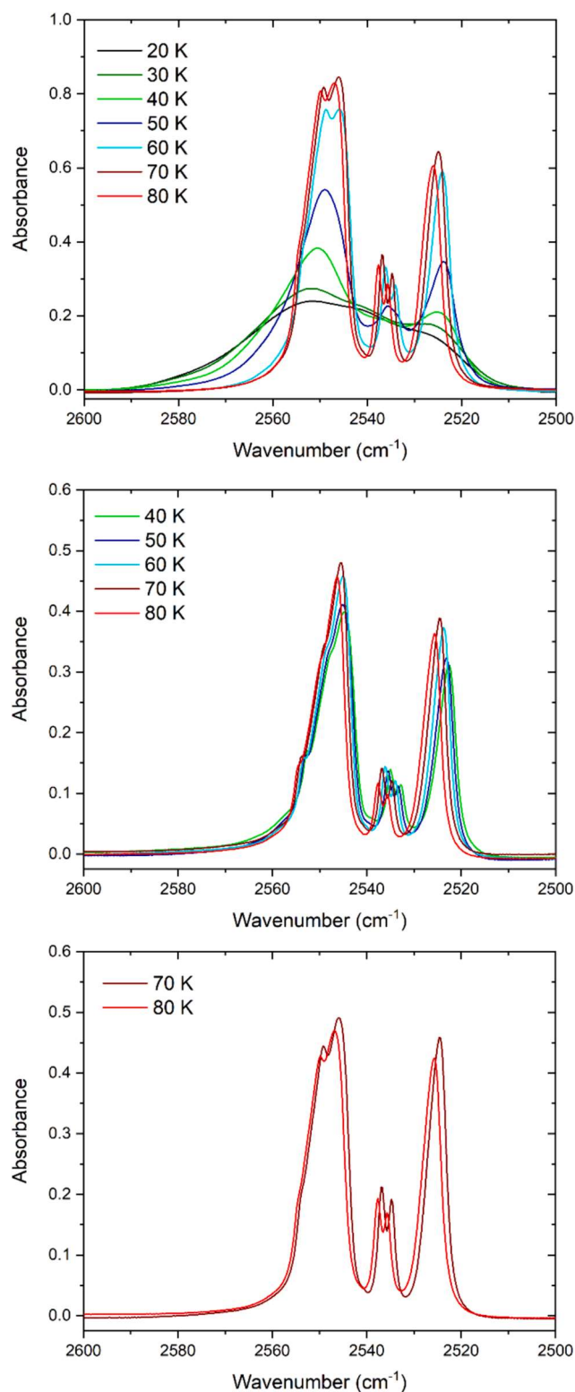
Fig. 2. Thermal evolution of the band attributed to the \text{H}_2\text{S} \nu_s modes for ices deposited at 20, 40, and 70 K. Note the readily observable presence of the individual \nu_3 , \nu_1 ( E_u ), and \nu_1 ( A_{2u} ) modes (in order from highest to lowest wavenumber position) in the crystalline ices.
