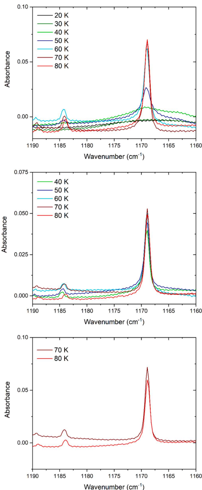
Fig. 4. Thermal evolution of the band attributed to the H 2 S \nu_2 modes for ices deposited at 20, 40, and 70 K. Note the readily observable presence of the individual \nu_2 ( E_u ), and \nu_2 ( A_{2u} ) modes (in order from highest to lowest wavenumber position) in the crystalline ices.
