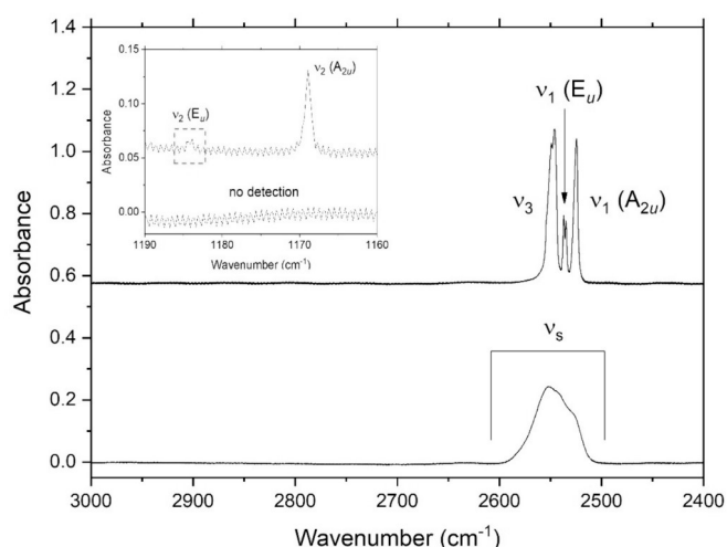
Fig. 1. Mid-infrared absorption spectra of amorphous (lower plot) and crystalline (upper plot) \text{H}_2\text{S} ices deposited at temperatures of 20 and 70 K, respectively. The estimated thicknesses of the amorphous and crystalline ices are 0.882 \pm 0.063 and 0.530 \pm 0.038 \mu\text{m} , respectively. Note that spectra are vertically offset for clarity. The inset depicts the weak band corresponding to the \nu_2 mode which is not visible in the spectrum of the amorphous ice.
