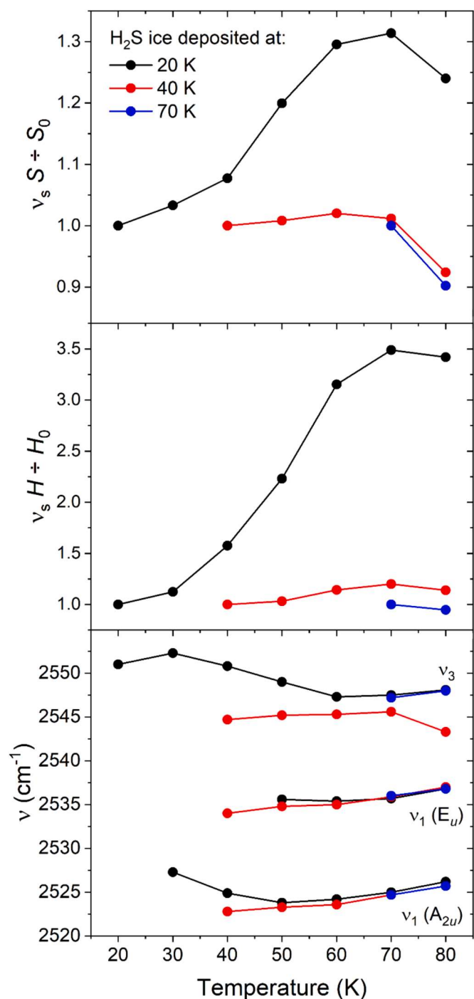
Fig. 3. Variations in the integrated absorbance S (top panel), peak height H (middle panel) and peak positions \nu (bottom panel) of the \nu_s modes for \text{H}_2\text{S} ices deposited at 20 (black circles), 40 (red circles), and 70 K (blue circles). Note that the variations in S and H are reported relative to their initial values S_0 and H_0 upon deposition of the ice. Error bars have been omitted for clarity, but upper bounds to the uncertainties associated with S / S_0 , H / H_0 , and \nu have been calculated to be \pm 7\% , \pm 15\% , and \pm 0.25 \text{ cm}^{-1} , respectively.
