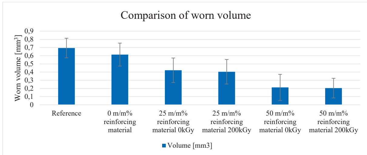
Figure 7. Comparison of wear volumes
