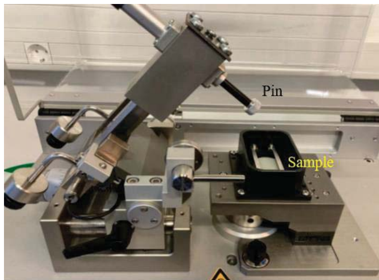
Figure 5. Pin-on-disk tribometer
