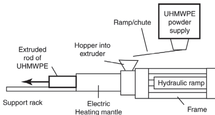
Figure 2. RAM extruder [2]
