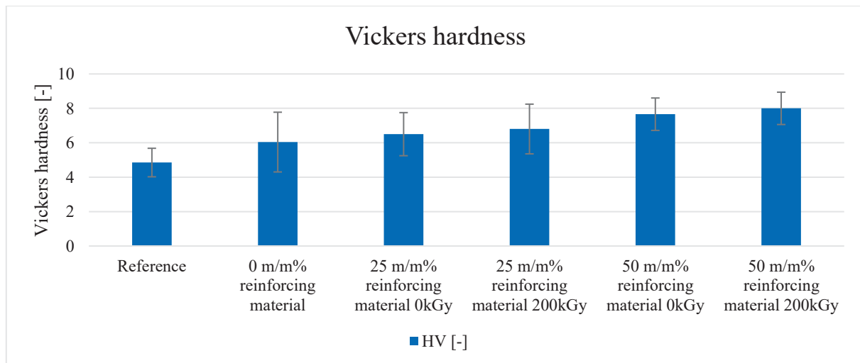
Figure 8. Comparison of Vickers hardness values
