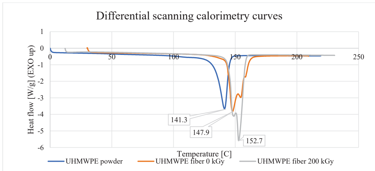
Figure 4. Melting point marked on differential scanning calorimetry curves
