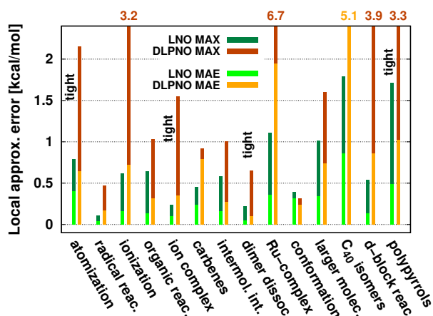
Fig. 8 Mean absolute error (MAE) and maximum error [in kcal/mol] of default (or when labeled explicitly, tight) LNO-CCSD(T) (left bars) and DLPNO-CCSD(T) (right bars) against canonical CCSD(T) for various energy difference properties. The average system size increases from left to right. MAE or MAX values above 2.2 kcal/mol are given at the top of the figure to improve visibility. The numerical values and additional details are collected in Table 4 and S1.
