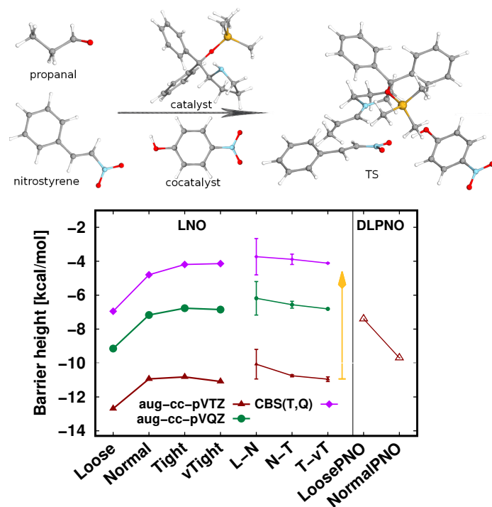
Fig. 7 Transition state barrier height of a organocatalytic Michael-addition reaction comparing LNO-CCSD(T) (left) and DLPNO-CCSD(T 1 ) (right) energies. 29
