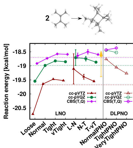
Fig. 5 Reaction energy of octamethylcyclobutane (OMCB) dimerized from 2,3-dimethylbut-2-ene of the NWH reaction compilation 30 . The plot shows LNO-CCSD(T) (left), LAF extrapolated LNO-CCSD(T) according to Eq. 5 (middle) and DLPNO-CCSD(T) 1 (right) results compared to the horizontal lines corresponding to the conventional CCSD(T) results. The Normal LNO-CCSD(T)/ \Delta CBS(T,Q) basis set correction to Normal – Tight LNO-CCSD(T)/haTZ in the composite E_{\text{LAF}}^{\text{CBS}(X,X+1),X} approach of Eq. 7 is depicted as an orange vertical arrow.
