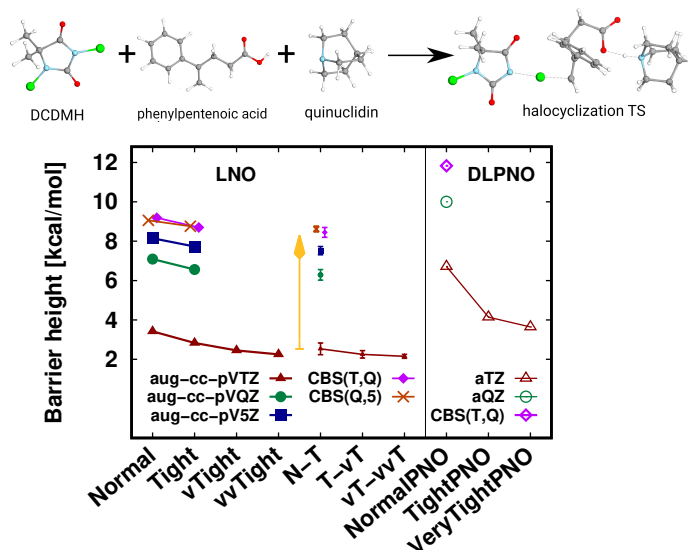
Fig. 6 Transition state (63 atoms) barrier height of a halocyclization reaction comparing LNO-CCSD(T) (left) and DLPNO-CCSD(T 1 ) (right) barrier height energies. 150,154 The CBS(T,Q) and CBS(Q,5) LNO-CCSD(T) results are slightly shifted along the x-axis to increase visibility.
