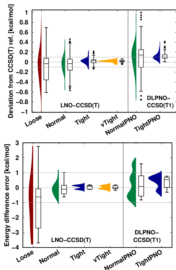
Fig. 9 LNO-CCSD(T) (left) and DLPNO-CCSD(T 1 ) (right) energy deviations against the DF-CCSD(T) reference for the S66 153 interaction energy compilation in the haug-cc-pVTZ basis set 149 (top panel) and the CEMS26 compilation 29 (bottom panel). (Half) violin curves show the distribution of the signed errors, where the height of the curve (along the horizontal axis) indicates the frequency of the signed errors corresponding to an error value on the vertical axis. The horizontal lines of the boxes indicate the lower, median, and upper quartiles, respectively. Whiskers extend to the most distant data point whose error value lies within 1.5 times of the difference between the lower and upper quartiles. Outliers beyond the whiskers, if any, are represented by dots. The numerical data is from Tables 3 and S2 of Ref. 29.
