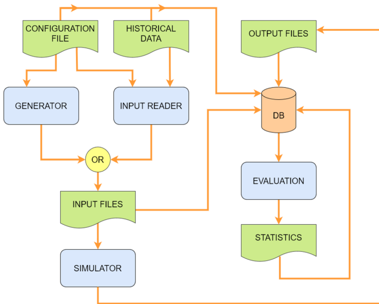
Fig. 1 Workflow of the ENCKEP simulator
