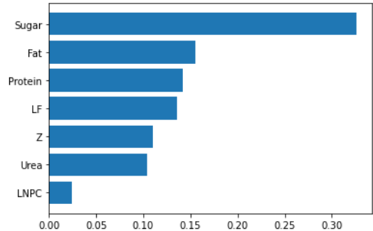
Figure 2. The result of the feature importance scoring for the best model’s input parameters.
