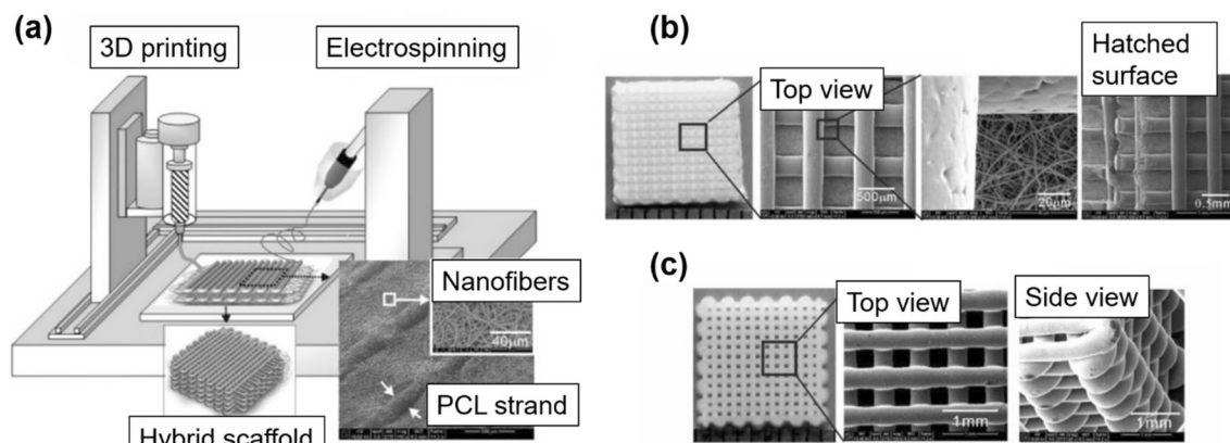
FIGURE 14 | (a) Schematic diagram illustrating the combination of ES and 3D printing techniques for creating ECM scaffold, (b) SEM images of hierarchical PCL scaffolds produced by integrating ES with 3D printing. (c) SEM images of PCL scaffolds were produced exclusively by the 3D printing technique [165]. Reproduced with permission from John Wiley and Sons.
