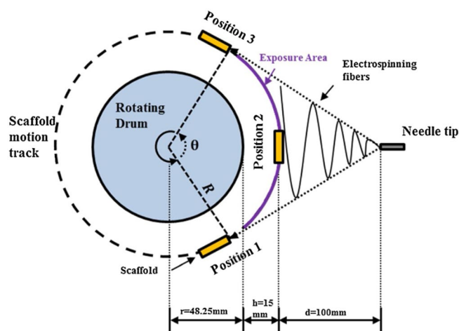
FIGURE 17 | Hybrid printing technique that integrates screw-assisted 3D printing with rotational ES. This figure is based on the work by Huang et al., titled Engineered dual-scale poly ( \epsilon -caprolactone) scaffolds using 3D printing and rotational electrospinning for bone tissue regeneration and is licensed under the Creative Commons Attribution 4.0 International License (CC BY 4.0). The original work can be found in reference [196].
