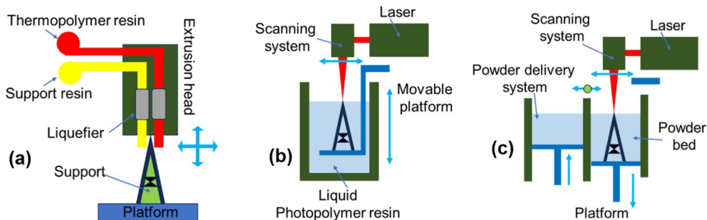
FIGURE 10 | Common 3D printing methods for scaffold fabrication (a) Fused filament fabrication (FFF), (b) Stereolithography (SLA), and (c) Selective laser sintering (SLS). This figure is based on the work by Z.-X. Low et al., titled Perspective on 3D printing of separation membranes and comparison to related unconventional fabrication techniques , and is licensed under the Creative Commons Attribution 4.0 International License (CC BY 4.0). The original work can be found in reference [125].
