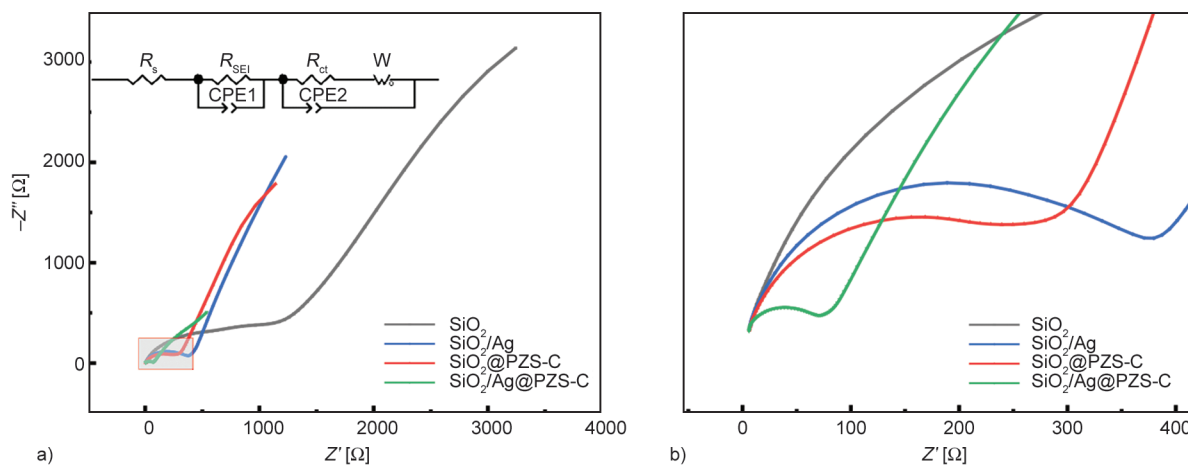
Figure 11. a) EIS spectrum of samples; b) zoomed-in view at the high-frequency region.
