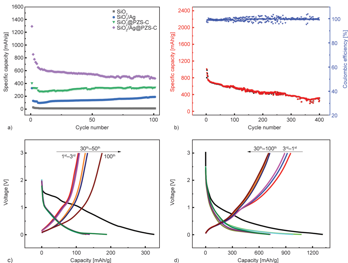
Figure 9. a) Cyclic performance of samples at 100 \text{ mA} \cdot \text{g}^{-1} current density; b) cyclic stability performance of \text{SiO}_2/\text{Ag}@ \text{PZS-C} ; Galvanostatic discharge/charge profiles of c) \text{SiO}_2/\text{Ag} and d) \text{SiO}_2/\text{Ag}@ \text{PZS-C} .
