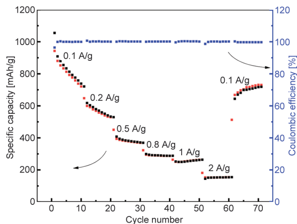
Figure 10. Rate performance of SiO 2 /Ag@PZS-C.
