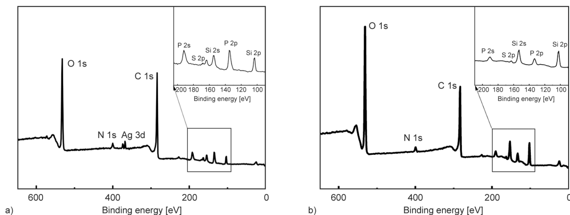
Figure 6. XPS spectra of prepared a) SiO 2 /Ag@PZS-C and b) SiO 2 @PZS-C.
