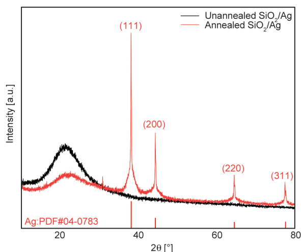
Figure 3. XRD spectra of \text{SiO}_2/\text{AgNO}_3 and \text{SiO}_2/\text{Ag} .
