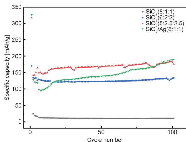
Figure 7. Lithium storage cycle performance of \text{SiO}_2 negative electrode (containing different proportions of conductive agent) and \text{SiO}_2/\text{Ag} .
