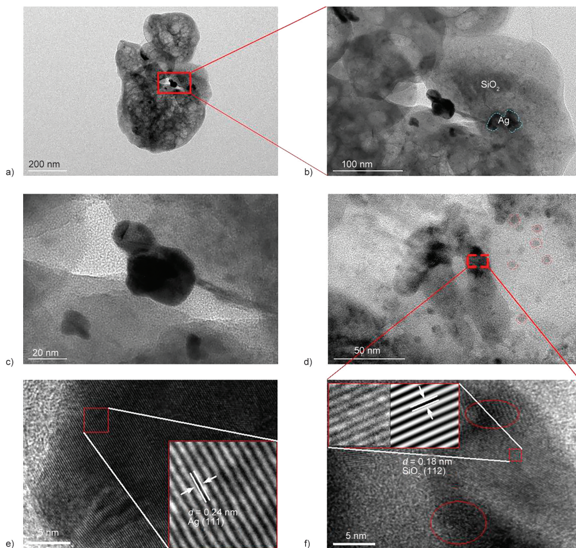
Figure 2. TEM images of \text{SiO}_2/\text{Ag}@PZS\text{-C} . In (f), the magnified image is embedded in the upper left corner, along with the Fourier transform analysis conducted using DigitalMicrograph. a) TEM image of sample with scale of 200 nm; b) TEM image of sample with scale of 100 nm; c) TEM image of sample with scale of 20 nm; d) TEM image of sample with scale of 50 nm; e), f) TEM images of sample with scale of 5 nm, and the magnified image is embedded in the corner, along with the Fourier transform analysis conducted using DigitalMicrograph.
