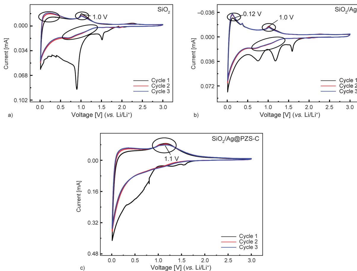
Figure 8. CV curves of a) SiO 2 , b) SiO 2 /Ag and c) SiO 2 /Ag@PZS-C.
