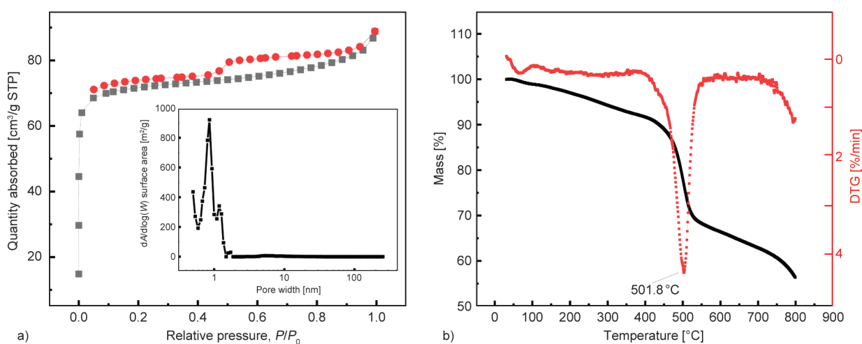
Figure 4. a) \text{N}_2 adsorption-desorption curve and pore distribution curve of \text{SiO}_2/\text{Ag}@PZS\text{-C} and b) thermogravimetric (TG)/differential thermogravimetric (DTG) curve of \text{SiO}_2/\text{Ag}@PZS\text{-C} .
