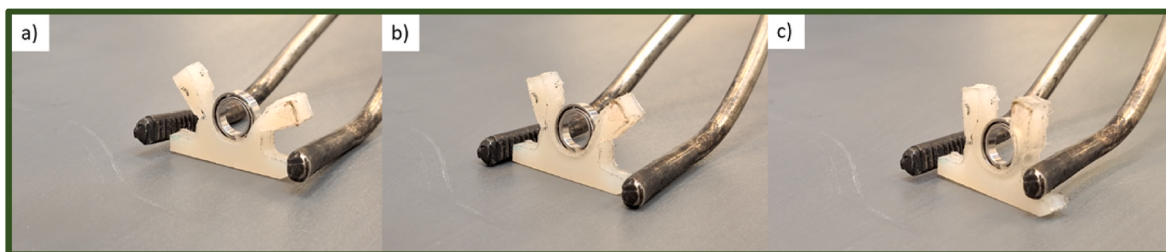
Fig. 9. Demonstration of shape memory on a bearing housing. Programmed shape (a), recovery process (b), and recovered shape (c).
